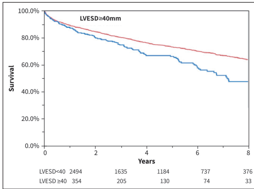
Figure 1. Survival stratified by LV size parameters.
