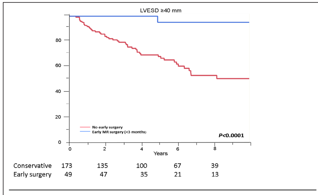
Figure 3. Survival stratified by early surgery (<3 months) in patients with moderate MR and LVESD \geq 40 mm or < 40 mm.
