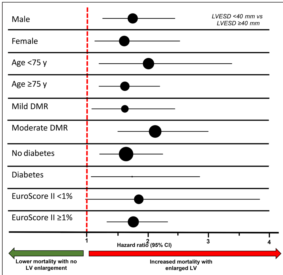
Figure 2. Forest plot of mortality under medical management.
