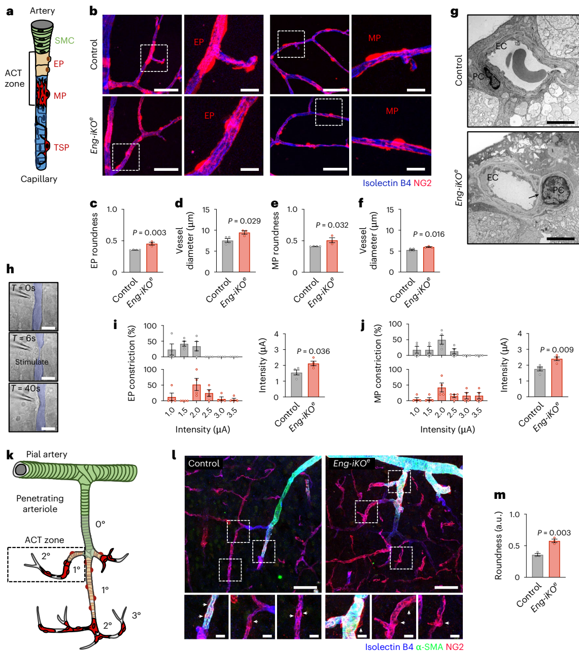
Fig. 1 | Mural cell organization in Eng-iKO e mouse retinal and cerebral vasculature. a , Schematic of mural cell populations along the arterial–capillary axis. b , Confocal images of genetically labelled retinal EPs and MPs (NG2DsRedBAC transgenic mice, red) attached to endothelium (isolectin-B4, blue) in control and Eng-iKO e mice. Scale bar, 50 \mu\text{m} . Higher magnification of EPs and MPs in boxes shown at right. Scale bar, 10 \mu\text{m} . c , Quantification of EP roundness and d , capillary diameters in control ( n = 3 , total pericytes = 67) vs Eng-iKO e ( n = 3 , total pericytes = 46) mice. e , Quantification of MP roundness and f , capillary diameters in control ( n = 3 , total pericytes = 95) vs Eng-iKO e ( n = 3 , total pericytes = 72) mice. g , TEM image of a retinal vessel with a contractile pericyte in Eng-iKO e mice. Scale bar, 2 \mu\text{m} . The black arrow indicates the basal membrane space located between an endothelial cell (EC) and a pericyte (PC). h , Vascular segment with a contractile pericyte before, during and after electrical
