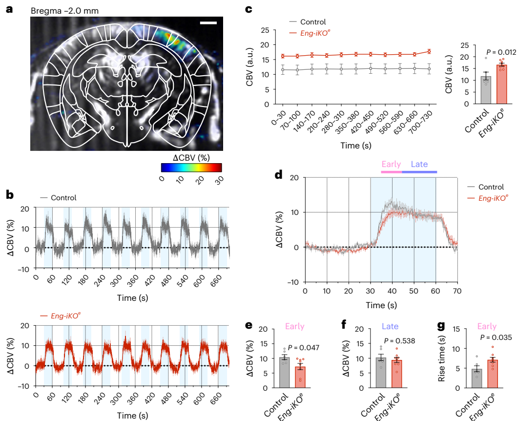
Fig. 4 | Neurovascular uncoupling revealed by fUS. a , Transcranial fUS imaging of task-induced changes in cerebral blood flow in the somatosensory cortex during whisker stimulation in anaesthetized mice. Scale bar, 1 mm. b , Mean time-series of all trials of the activated region, with blue boxes showing temporal correlation between the stimulus pattern and the haemodynamic response in both control ( n = 6 ) and Eng-ikO o ( n = 8 ) mice. c , Baseline CBV values over time
