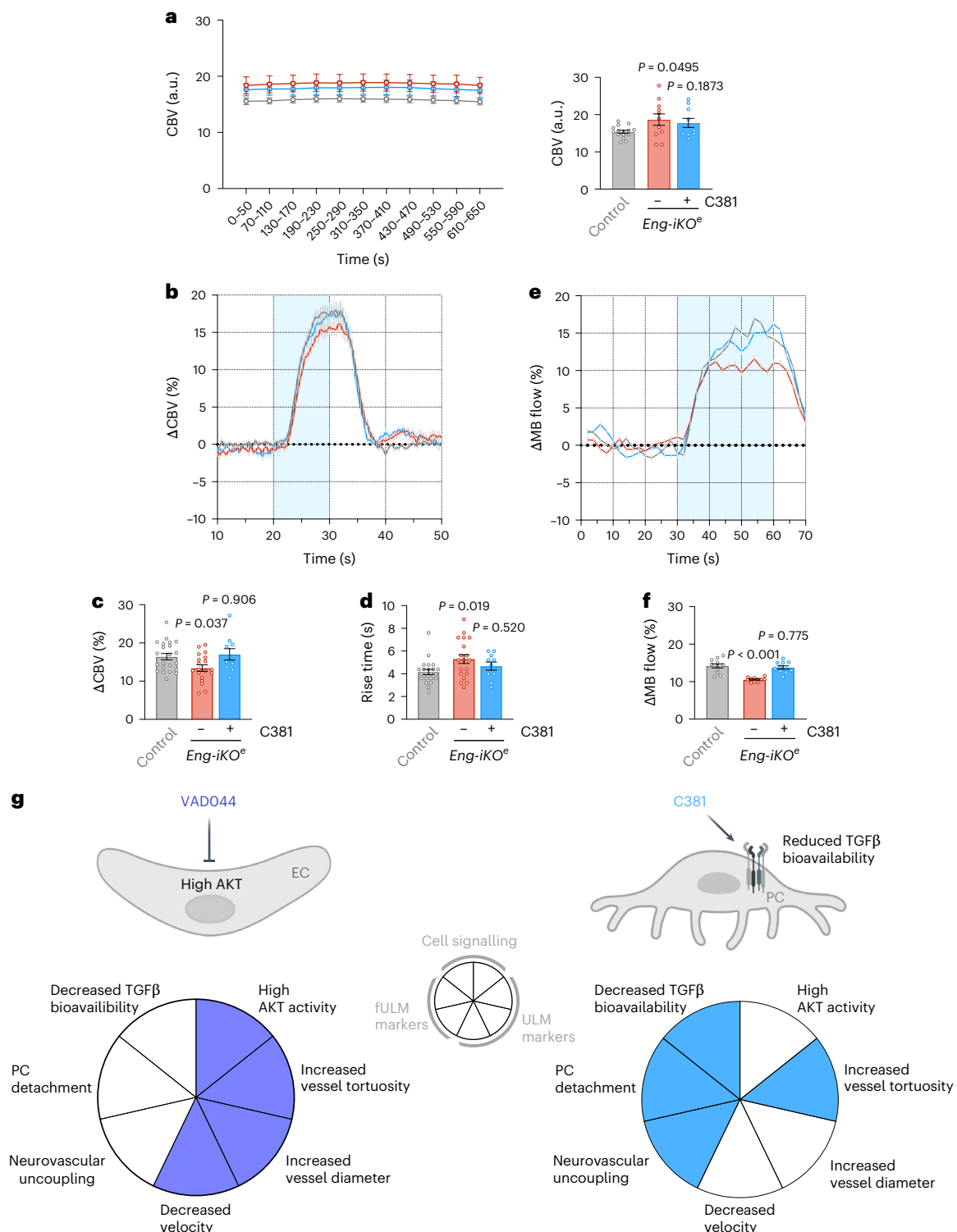
Fig. 8 | C381 drug restores haemodynamic response. a , Quantification of the baseline CBV in control ( n = 15 ), Eng-iKO e ( n = 11 ) and Eng-iKO e mice treated with C381 ( n = 10 ). b , Average of the haemodynamic response within a chosen region of interest in control ( n = 15 ), Eng-iKO e ( n = 11 ) and Eng-iKO e mice treated with C381 ( n = 10 ). c,d , Quantification of the increased response amplitude ( c ) and of the rise time ( d ) was performed in control ( n = 15 ), Eng-iKO e ( n = 11 ) and Eng-iKO e
