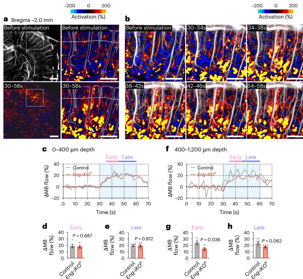
Fig. 5 | Contractile pericyte dysfunction during the hyperaemic response revealed by fULM. a , Top left, MB count ULM map at bregma = -2 mm containing the barrel cortex. Bottom left, corresponding fULM activation map showing the activated region in the barrel cortex. Scale bar, 1 mm. Top right, zoom-in of the fULM activation map showing the absence of hyperaemia before stimulation in the 24–28 s time window. Scale bar, 500 μm. Dashed white line corresponds to z = 400 μm depth in the cortex. Bottom right, zoom-in of the fULM activation map during the stimulation (30–58 s). Scale bar, 500 μm. b , Activation maps and MB tracks detected in 4-s
