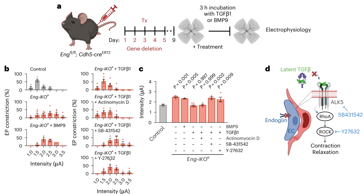
Fig. 6 | Impaired TGF \beta bioavailability in Eng-iKO e mice. a , Schematic showing adult induction of Eng deletion in endothelial cells and ex vivo retina treatments. Tx, tamoxifen b , Proportion of EPs inducing a vascular constriction at the indicated current ( \mu A) and c , mean intensity inducing EP-mediated vessel constriction in the different conditions. At day 9, retinas of Eng-iKO e mice were collected and incubated for 3 h in medium containing TGF \beta 1 (5 ng ml -1 ) ( n = 5, total EPs = 30) or vehicle alone ( n = 5, total EPs = 26) in the absence or presence of actinomycin D (1 \mu g ml -1 ) ( n = 4, total EPs = 21), SB431542 (10 \mu M) ( n = 3, total EPs = 15) or Y27632 (100 \mu M) ( n = 4, total EPs = 22) that inhibits the transcription, ALK5 or ROCK, respectively. Pericytes were then subjected to electrical
