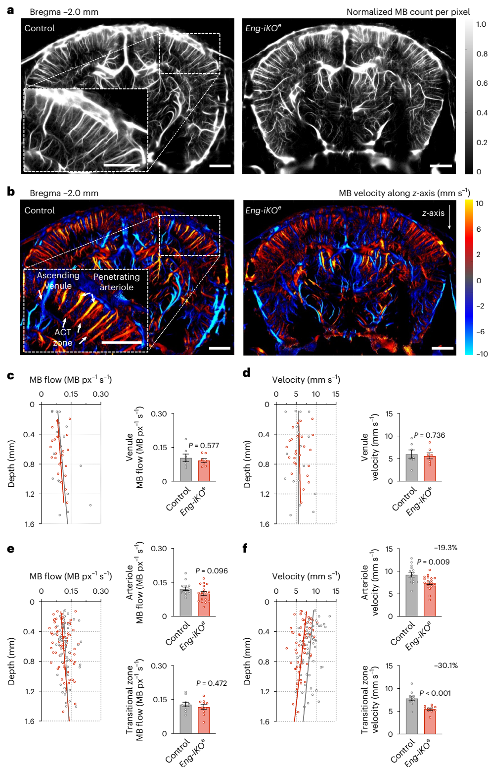
Fig. 2 | ULM reveals cerebral arteriole abnormalities in Eng-ikO e mice.
