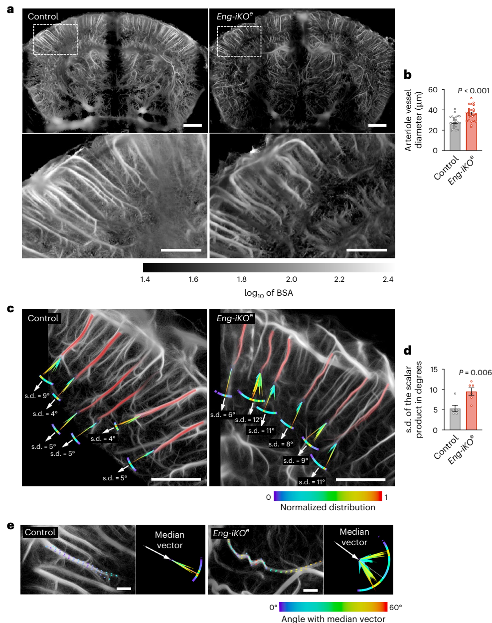
Fig. 3 | Analysis of the arteriolar architecture. a , ULM backscattering imaging offering better blood vessel delineation than MB count. Scale bars, 500 \mu\text{m} . Higher magnification images of the cortex in boxes are shown at the bottom. Scale bar, 500 \mu\text{m} . b , Quantification of arteriolar blood vessel diameter in a control mouse ( n_{\text{vessel}} = 25 ) and in an Eng-iKO e mouse ( n_{\text{vessel}} = 25 ). c , High magnification images of MB count maps showing vessel tortuosity.
