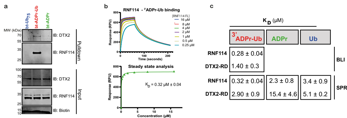
Fig. 2 | DTX2 and RNF114 interact with ADPr-Ub. a Cell lysate from HEK293T cells was incubated with biotin-ADPr-Ub probe 1 , biotin-Ub 75 and biotin-ADPr (5 \mu\text{M} ) and a pull down using Neutravidin beads was performed. Western blot shows levels of endogenous DTX2 and RNF114 (input) and pull-down confirms interacting with probe 1 . Source data are provided as a Source Data file. Representative blots for
