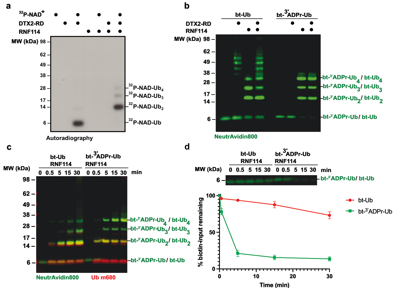
Fig. 3 | RNF114 elongates Ub chain on ADPr-Ub. a ^{32}\text{P-NAD}^+ -Ub formation assay with DTX2-RD and RNF114. RNF114 elongates Deltex-catalysed ^{32}\text{P-NAD}^+ -Ub. b Ubiquitination assay using biotin-Ub and biotin-ADPr-Ub probe 1. RNF114 elongates the Ub chain on biotin-Ub and biotin-ADPr-Ub probe 1. c RNF114 elongates Ub chains in a time-dependent manner. Biotin signal is shown in green, and ubiquitin signal is
