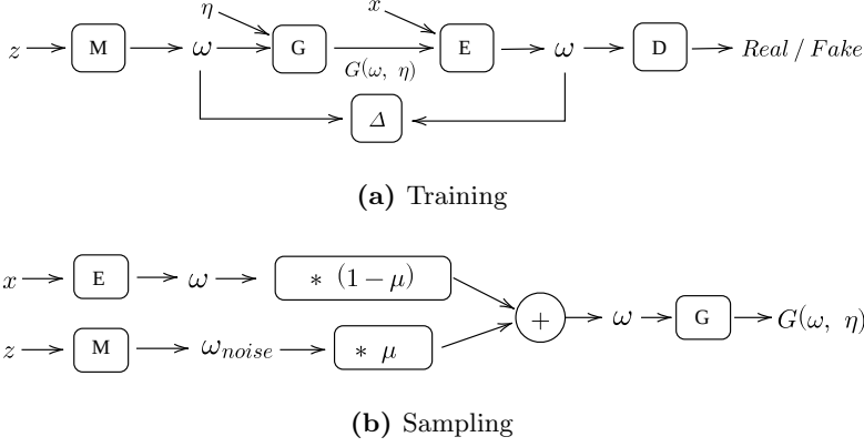
Figure 6.4: SA-ALAE in directed graphs. ALAE and SA-ALAE share an identical training strategy. The sampling procedure of SA-ALAE utilizes the off-the-shelf mapper M to sample additional noisy latent variables \omega_{noise} , hereby introducing randomness in the sampling.
