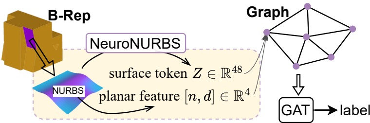
Figure 5.5: NURBS-GAT diagram.
