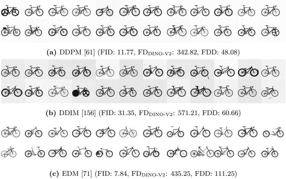
Figure 3.8: Qualitative evaluation of generated bicycle designs. DDPM and DDIM yield structurally more plausible results than EDM, but FID and FD_{DINO-V2} fail to agree with human judgments, whereas our FDD ranks the models with the perspective of structural plausibility and penalizes the visual artifacts as well.
