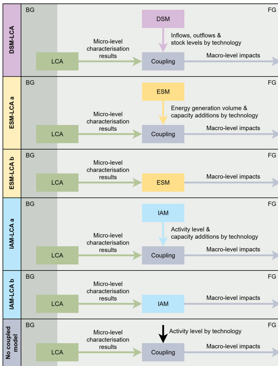
Fig. 2 Stylised Overview of main modelling approaches in prospective macro-level Life Cycle Assessment (LCA), grouped by how the foreground (FG) system was scaled to macro-level: coupling process-based LCA with a Dynamic Stock Model (DSM-LCA), an Energy System Model (ESM-LCA), an Integrated Assessment Model (IAM-LCA), or without a coupled model. Labels ‘a’ and ‘b’ indicate whether the combination is applied ex-post (after running the ESM or IAM) or endogenously (with micro-level LCA characterisation results directly embedded). Coupling is illustrated in the FG system; background (BG) system couplings (e.g., via premise (Sacchi et al. 2022) are not shown. Note that the characterisation results can be either integrated over time for the whole life cycle or separated by life cycle stage. For ESM- and IAM-LCA approaches, we distinguish two modelling variants; see below for explanation. The diagrams reflect generalised structures; individual studies may differ
