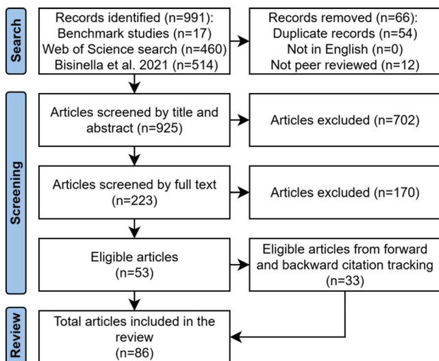
Fig. 1 Summary of the literature selection process, adapted from Page et al. (2021) and based on the recommendations of Siddaway et al. (2019). A complete list of retrieved articles, including reasons for exclusion, is provided in the Supplementary Information
