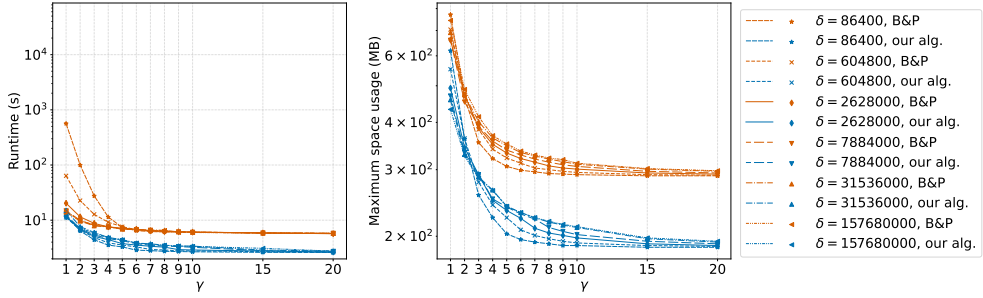
(b) Facebook-wosn-wall
