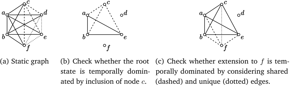
Figure 4.8: Bulking phase branch cut example
