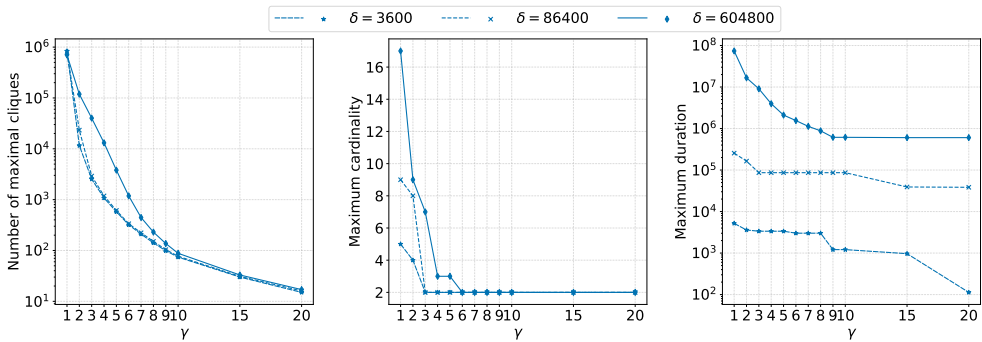
(c) Reddit Hyperlinks
