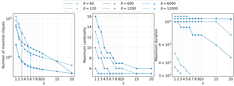
(a) Infectious I
