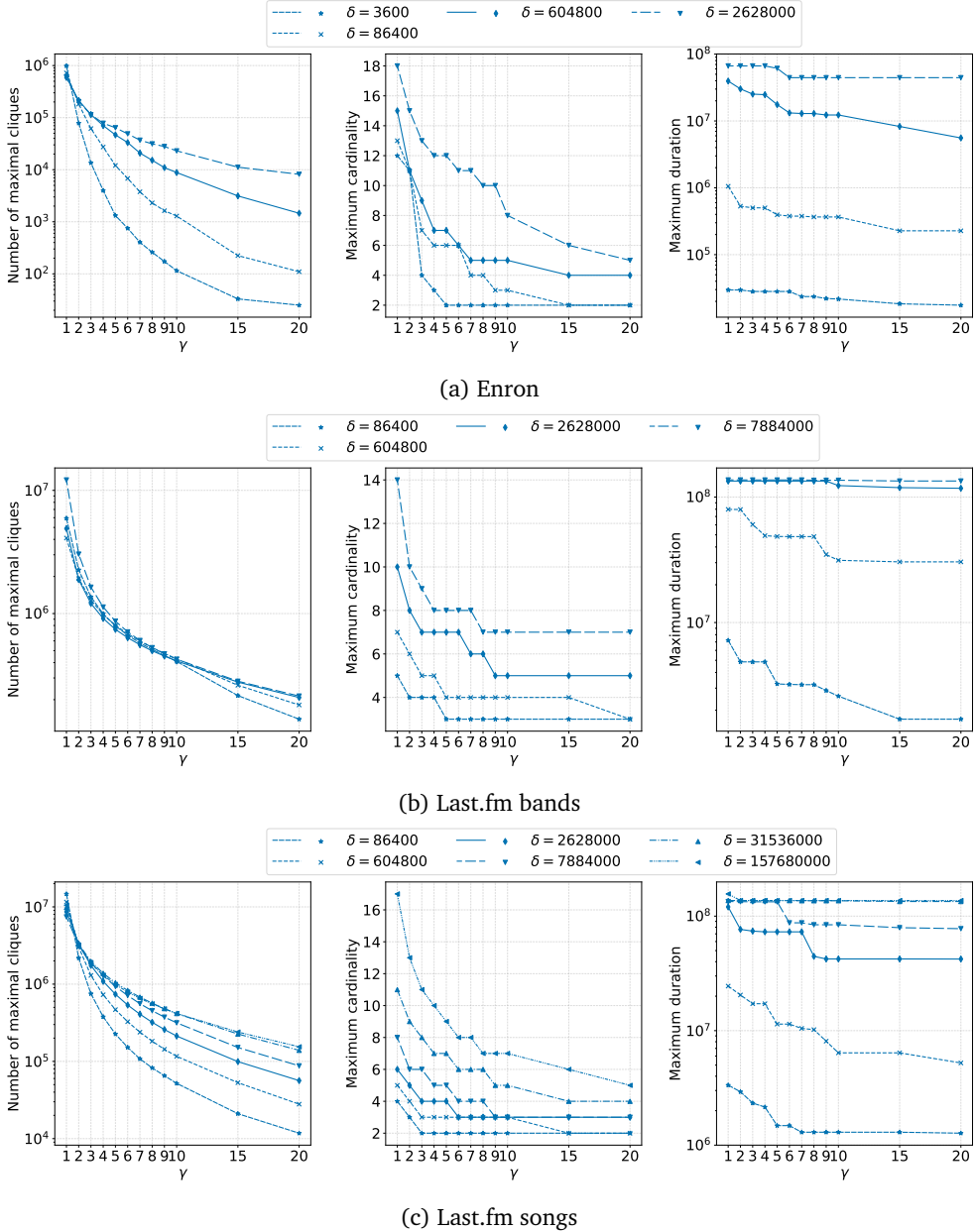
Figure 4.18: Properties of the set of enumerated cliques for a range of \gamma values. The left panels show the number of (\delta, \gamma) -maximal cliques found and the middle and right panels show, respectively, their maximum cardinality and maximum duration.
