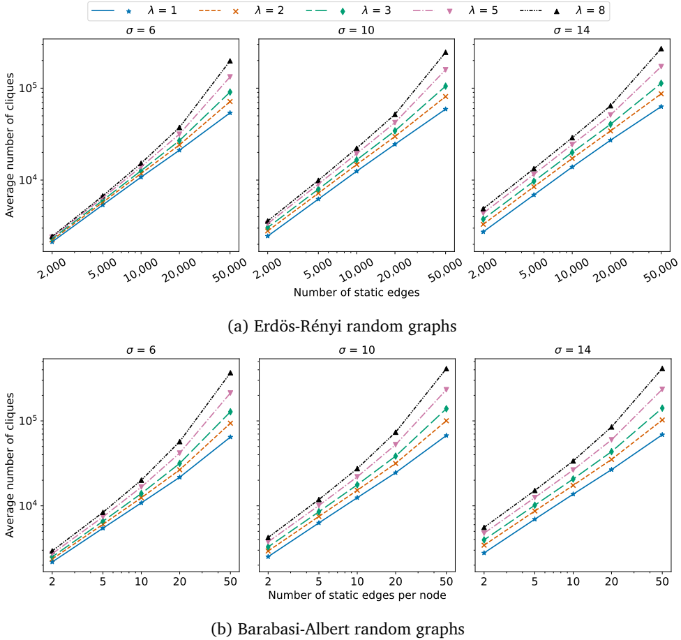
Figure 4.9: Average number of (\delta, \gamma) -maximal cliques for each density parameter setting.
