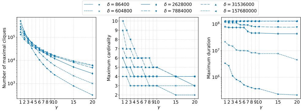
(b) Facebook-wosn-wall
