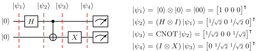
Fig. 1. An example 2-qubit quantum circuit. Each qubit is represented by a horizontal wire, and operations are applied from left to right. As is common, we write |xy\rangle as shorthand for |x\rangle \otimes |y\rangle . Measuring both qubits after obtaining |\psi_4\rangle = 1/\sqrt{2}(|01\rangle + |10\rangle) gives |01\rangle or |10\rangle each with probability |1/\sqrt{2}|^2 = 1/2 .
