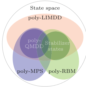
Fig. 3. The comparative succinctness of LIMDD, QMDD, MPS, and RBM (see Sect. 7) following from the asymptotic analysis in [177]. All these data structures, except the stabilizer formalism, can represent any quantum state (they are universal). The Venn diagram however shows families of states that can be represented in polynomial size with the different data structures. Consequently, MPS, RBM, and LIMDD are incompatible in terms of representation power: they each have their strengths and weaknesses. LIMDD is the only structure that can represent all stabilizer states and all (families of) states supported by polynomial QMDD. (Poly-)ADD and QuiDD are not shown but are strictly contained in (Poly-)QMDD.
