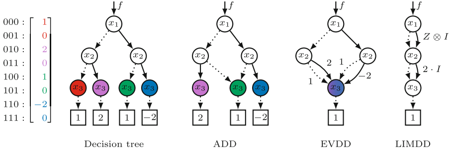
Fig. 2. A pseudo-Boolean function f(x_1, x_2, x_3) = \overline{x_3} \cdot (2 \cdot x_2 \cdot (\overline{x_1} - x_1) + \overline{x_2}) represented as (non-normalized quantum state) vector and as an (exponentially-sized) decision tree. A node labeled with variable x represents a Shannon decomposition on x . An outgoing dashed edge represents the sub-functions where the variable x is restricted to false (0) and a solid edge where the variable is restricted to true (1). The boxes represent leaves. We omit zero leaves. From a decision tree to algebraic decision diagram (ADD): The red node is merged into the green as both represent the same sub-function f_{00}(x_3) = f_{10}(x_3) = 1 - x_3 . From algebraic decision diagram to edge-valued decision diagram (EVDD): The purple, green, and blue nodes represent sub-functions that are equivalent up to a constant factor of 2, 1, -2 respectively. By putting the factors on the edges, these equivalent nodes can be merged. Unlabeled edges have implicit factor 1. From edge-valued decision diagram (EVDD) to LIMDD: The Pauli LIM Z \otimes I maps f_0 to f_1 (as vectors, i.e. (Z \otimes I) \cdot [f_{100} \ f_{101} \ f_{110} \ f_{111}]^T = [f_{100} \ f_{101} \ -f_{110} \ -f_{111}]^T = f_0 ). Both x_2 nodes can thus be merged by putting this map on the (high) edge. Unlabeled edges to nodes x_i have implicit map 1 \cdot I^{\otimes i} .
