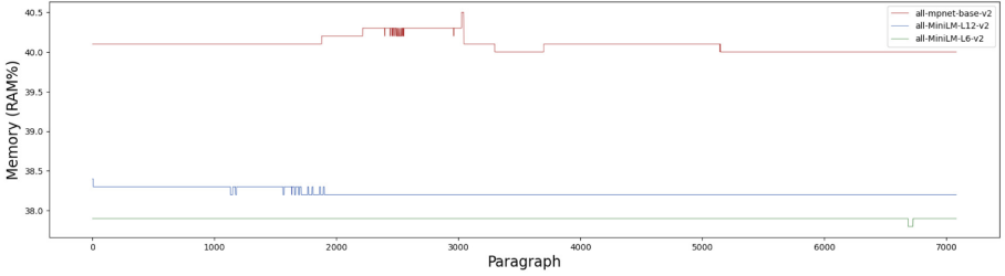
Fig. 7. RAM% consumed to create SBERT embeddings per paragraph.
