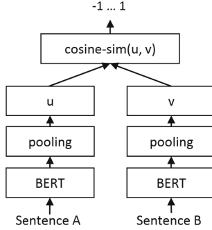
Fig. 1. Simplified architecture of SBERT [19].
