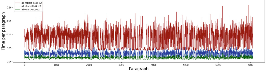
Fig. 6. Time consumed to create SBERT embeddings per paragraph.
