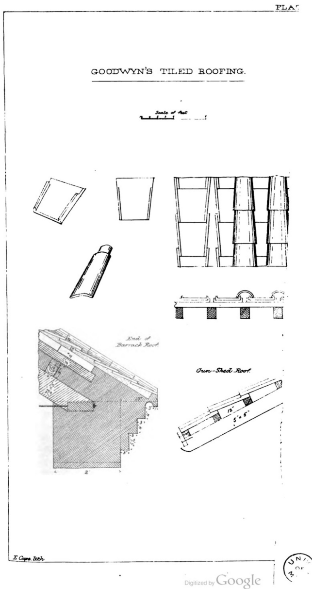
Figure 10.11: Goodwyn tiles drawing. Source: Professional Papers on Indian Engineering. 26
