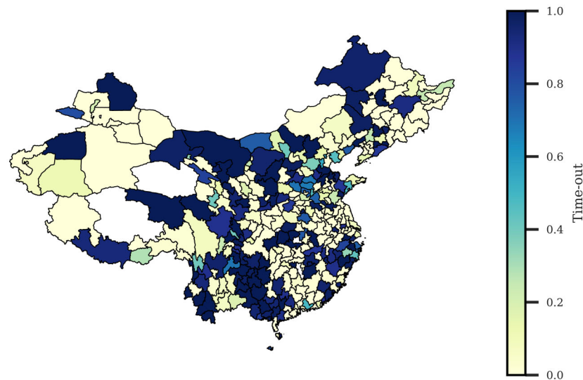
Figure 3 Proportion of websites that time-out relative to total number of tested websites, categorized by their corresponding prefecture-level division. Testing location: USA, Los Angeles.
