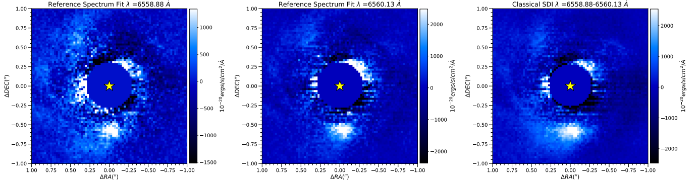
Figure 2. Other MUSE reductions showing the detection of AB Aur b from OB4. (Left and middle) 6558.88 Å and 6560.13 Å from the reduction shown in Figure 1. Average of the 6558.88 Å and 6560.13 Å slices from a classical SDI reduction (right). In each panel, we mask the field out to a separation affected by horizontal striping and saturation.
