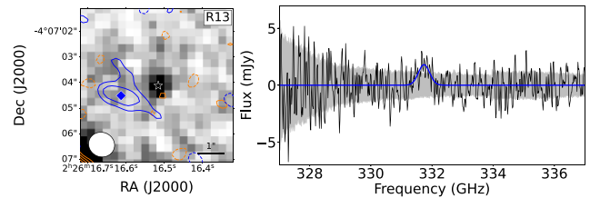
Figure B1. Left: the \text{SNR}_{\text{MF3D}} = 5.35\sigma peak that is found 1.45 arcsec from the center of the observations of REBELS-13. The potential [O\text{ III}]_{88\mu\text{m}} emission is plotted with blue contours and the corresponding beam of the moment-0 map is shown. The diamond indicates the peak emission in the moment-0 image, the star shows the peak of the rest-UV emission and the orange contours show the dust continuum emission. The contours run from 2\sigma to 5\sigma (in steps of 1\sigma ) and negative contours are shown with dashed lines. Right: the spectrum obtained with a circular aperture with 1 arcsec radius at the position of the peak with the 1\sigma uncertainty determined from 1000 random apertures. Due to the low significance of the peak in the spectrum and the large offset from the rest-UV position we interpret it as a probable noise feature.
