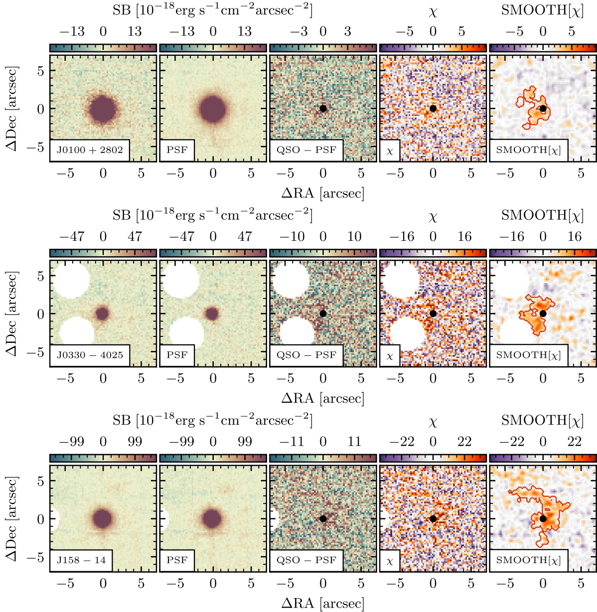
Figure 1. Quasars in our sample with extended nebular emission. From left to right, the panels display pseudonarrowband images of (1) the quasar’s Ly \alpha , (2) the PSF extracted from the broad wing of the quasar’s Ly \alpha line, (3) the PSF-subtracted data, (4) the \chi data, essentially representing the SNR of the PSF-subtracted data, and (5) the smoothed \chi data showing the extended nebular emission. Panels (1), (3), (4), and (5) are collapsed across the wavelength range of the detected nebula, and panel (2) is collapsed across the wavelength range of the PSF extraction, as displayed in Appendix B. White patches correspond to masked foreground sources.
