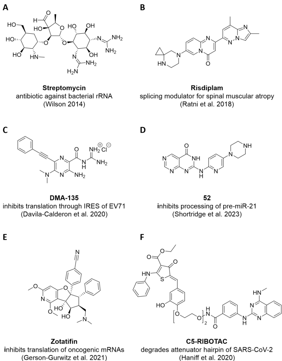
Figure 1.4. Chemical structures of small molecules targeting bacterial, viral or human RNA.
