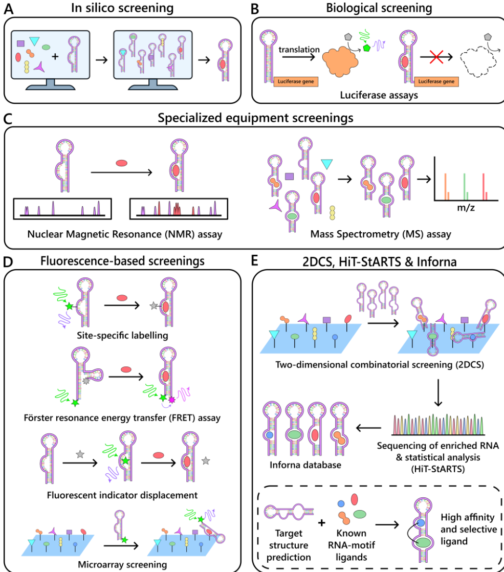
Figure 1.5. High-throughput screening methods for targeting RNA with small molecules. A) In silico screening. B) Biological screening with luciferase assays. C) Specialized equipment screenings, with for example nuclear magnetic resonance (NMR) and mass spectrometry (MS) assays. D) Fluorescence-based screening methods, such as site-specific fluorescent labelling, Förster resonance energy transfer (FRET), fluorescent indicator displacement and microarray screenings. E) Screening with the Inforna database, which was created by two-dimensional combinatorial screening (2DCS) followed by sequencing of enriched RNA & statistical analysis (HiT-StARTS). The Inforna database contains motif-specific ligands that can be combined to form high affinity and selective ligands.
