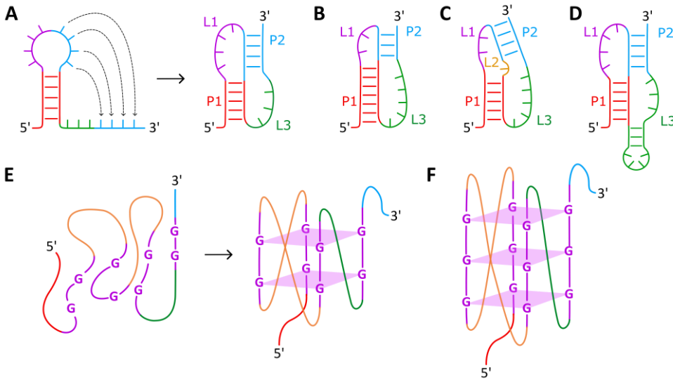
Figure 1.3. A) Folding of a hairpin (H)-type pseudoknot (PK). Indicated are stem 1 (P1), loop 1 (L1), stem 2 (P2) and loop 3 (L3). B) PK with different stem and loop lengths. C) PK with loop 2 (L2) between stacked helices and a varying relative angle between the helices. D) PK with a secondary structure in L3, called a HL_{out} PK. E) Folding of a two-tetrad G-quadruplex. Guanine tetrads are indicated in purple. F) A three-tetrad G-quadruplex.
