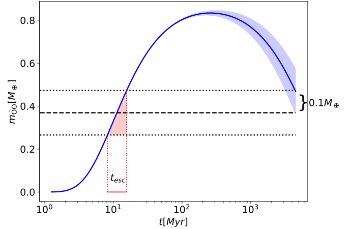
Fig. 2. Reconstruction of the time when the Sun left the parent cluster for a specific set of parameters. The dark blue curve shows the Öpik-Oort cloud’s mass-evolution, assuming it was born in isolation (fast-rise-exponential-decay function with a maximum mass of \mu_{\text{ÖO}} = 0.027 , t_{\text{rise}} = 10 Myr, and t_{\text{decay}} = 7500 Myr, see Eq. (E.1)). The blue-shaded area gives the uncertainty of the Öpik-Oort cloud for t_{\text{decay}} = 5000 Myr to 10\,000 Myr (see also Fig. 3 in the main paper). The dashed line indicates 0.38 M_{\oplus} below the endpoint of the solid blue curve. The intersections between the dashed line and the solid blue curve (to the left) indicate the moment the Sun left the parent cluster at t_{\text{esc}} = 12 \pm 4 Myr. The horizontal dotted lines are identical to the dashed line, but present the extremes for the blue-shaded region; they define the uncertainty in t_{\text{esc}} , indicated in red.
