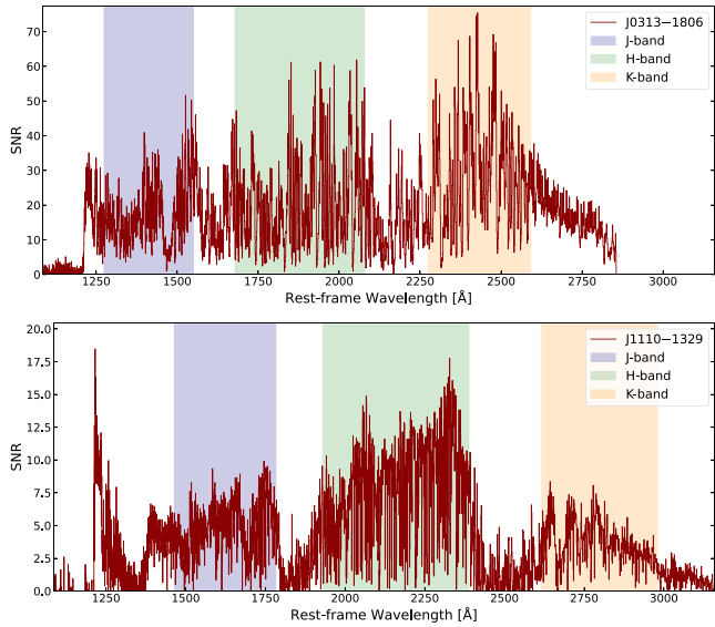
Figure C1. Top: example case of the distribution of the SNR along the wavelength grid [1040, 3332]\text{\AA} for the highest z quasar in the sample, J0313–1806 (dark red). The bands ( J , H , and K ) in which we compute the SNR are indicated according to different colours. Bottom: same, but for the lowest z quasar of the sample: J1110–1329.
