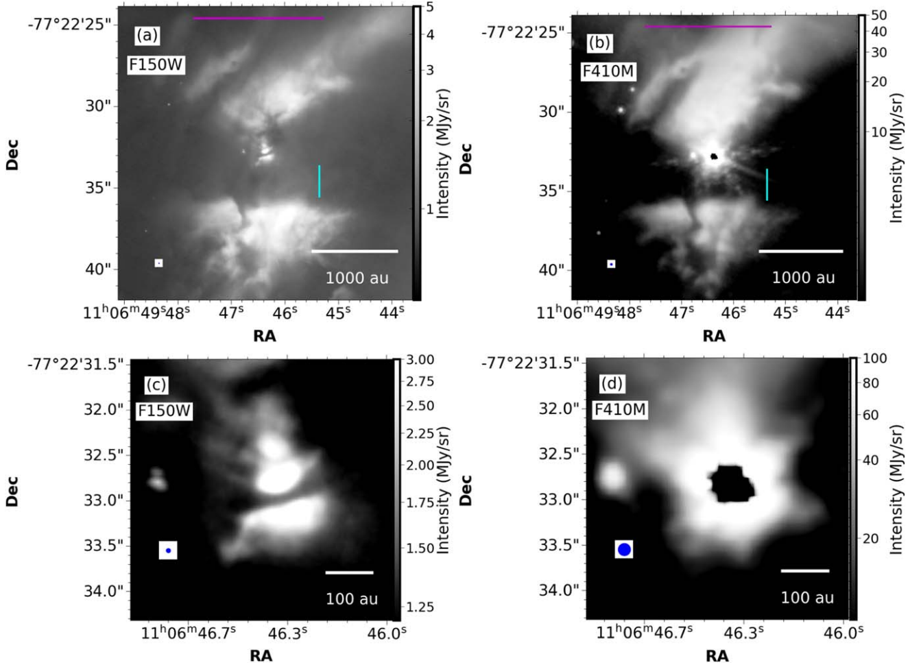
Figure 1. The NIRCам F150W and F410M filter image of the Ced 110 IRS4 region in gray scale. The NIRCам FWHM is shown in the lower left corner in blue. The scale bar in white is also shown in the lower right corner. The beam sizes are given in Table 2. The arc-like structure is marked with a magenta line, and the dark band is marked with a cyan line. The same intensity scaling is followed in Figure 2 for the NIRCам observations.
