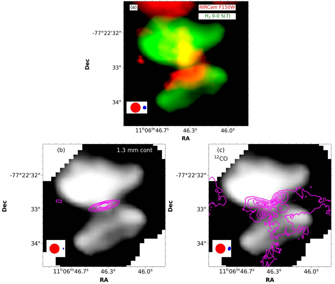
Figure 13. The molecular \text{H}_2 0–0 S(7) line with the NIRCам F150W emission, the SBLB 1.3 mm ALMA continuum, and the ALMA ^{12}\text{CO} observations. The MIRI FWHM based on D. D. Law et al. (2023) is shown in the lower left corner as a red circle, while the NIRCам/ALMA beam is shown as a blue ellipse.
