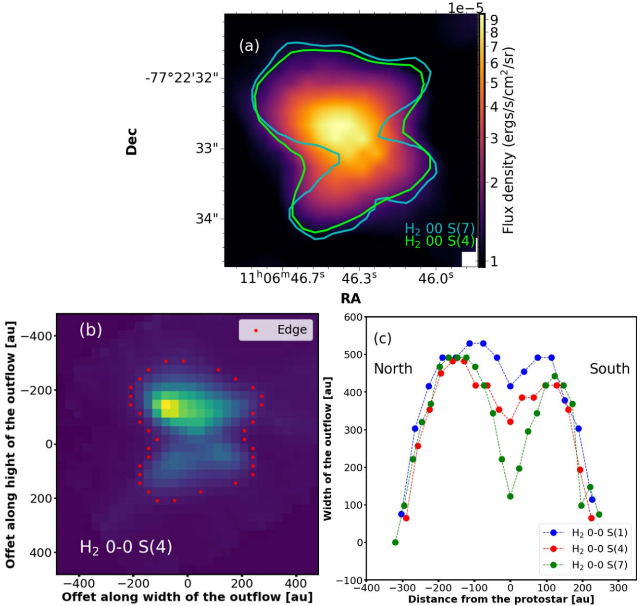
Figure 14. (a) The molecular \text{H}_2 0–0 S(1) line, with contours of 0–0 S(4) and 0–0 S(7) overlaid on top. The \text{H}_2 0–0 S(4) and \text{H}_2 0–0 S(7) contours are at 10% of the peak flux density ( 3.55 \times 10^{-4} \text{ erg s}^{-1} \text{ cm}^{-2} \text{ sr}^{-1} and 8.5 \times 10^{-4} \text{ erg s}^{-1} \text{ cm}^{-2} \text{ sr}^{-1} , respectively) of the emission. (b) The edge detected (in red) on top of the \text{H}_2 0–0 S(4) in color scale. (c) The outflow width as a function of distance from the protostar for the three ( \text{H}_2 0–0 S(1), S(4), and S(7)) transitions.
