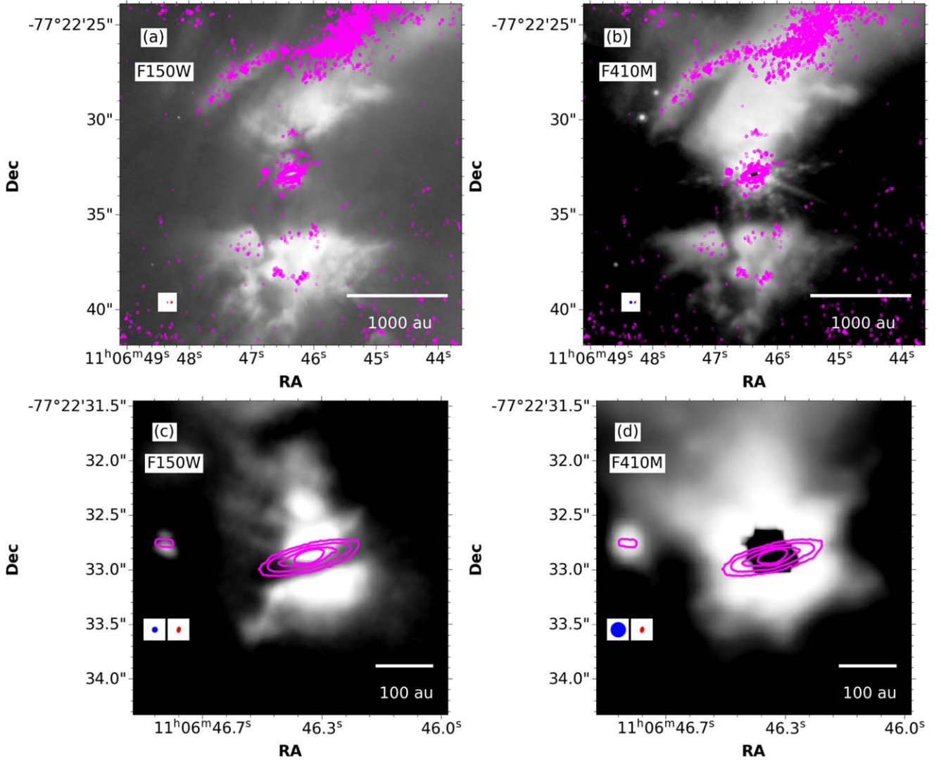
Figure 2. The NIRCам F150W and F410M filter image of the Ced 110 IRS4 region in gray scale is shown, with the ALMA 1.3 mm continuum map overlaid as magenta contours. The 1.3 mm continuum maps, with robust parameters of 2.0 and 0.0, are overlaid on the wide and zoomed-in views of the NIRCам image, respectively. The contours are 3\sigma , 10\sigma , 30\sigma , 70\sigma , and 100\sigma , with \sigma_{\text{robust}=2} = 14 \mu\text{Jy} and 10\sigma , 30\sigma , 70\sigma , and 100\sigma with \sigma_{\text{robust}=0} = 16 \mu\text{Jy} . The NIRCам FWHM and the ALMA beams are shown in the lower left corner as blue and red ellipses, respectively. The scale bar in white is also shown in the lower right corner. The beam sizes and PA are given in Tables 1 and 2.
