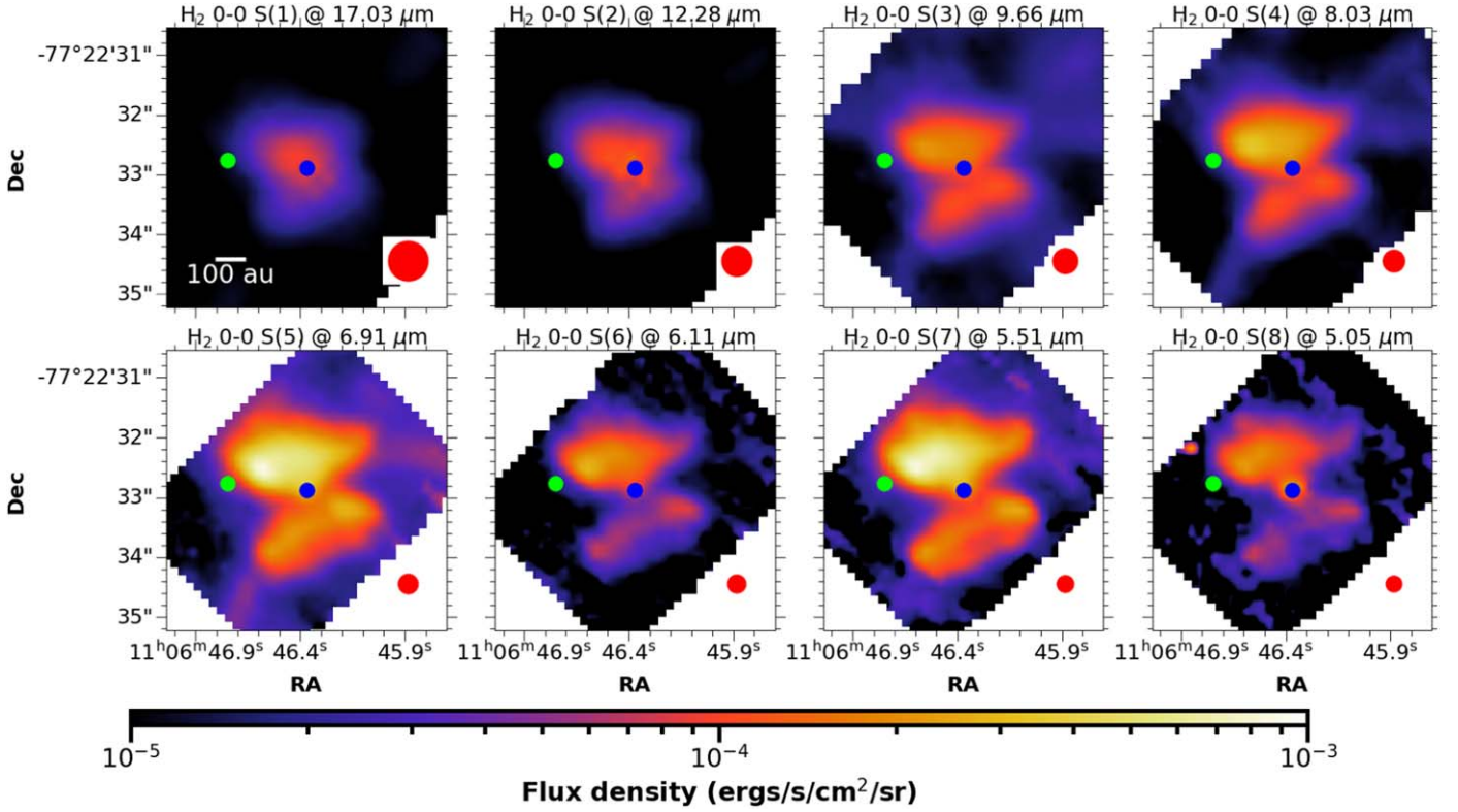
Figure 12. The morphology of the H 2 0–0 S line from S(1) to S(8) covering the MIRI MRS. All images are cropped to the same spatial scale of 5''.7 \times 5''.7 and have the same color scale. The ALMA 1.3 mm position for Ced 110 IRS4A is shown as a blue circle, and that for IRS4B is shown as a lime circle. The scale bar corresponding to 100 au is shown in the lower left corner. The MIRI FWHM based on D. D. Law et al. (2023) is shown in the lower right corner as a red circle.
