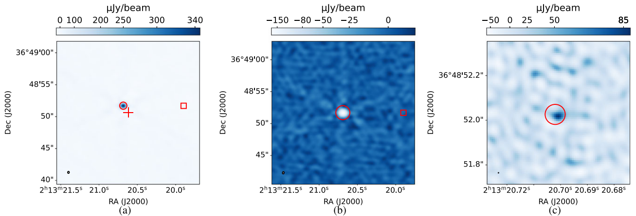
Figure 1. (a) Stokes I image of 2M0213 AB. The binary is unresolved and enclosed in the large circle. The binary is detected at a peak flux density of \sim 356 \mu\text{Jy beam}^{-1} . The 1\sigma r.m.s noise in the image is \sim 10 \mu\text{Jy beam}^{-1} giving a \text{SNR} \sim 36 . The binary at the true coordinates at epoch 2017-11-15 is offset from the pointing centre by \sim 1.3 arcsec, that is, by \sim 2 synthesized beamwidths due to proper motion effects described in Section 4.1. The position of the wide T3 brown dwarf companion at a separation \sim 16.4 arcsec is marked by the square box. The cross indicates the correlation centre (pointing centre). (b) Stokes V image of 2M0213 AB. The binary is unresolved and enclosed in the circle with a red outline. The data has been phase-shifted to the true coordinates at epoch 2017-11-15. The binary is detected at a peak flux density of \sim -174 \mu\text{Jy beam}^{-1} where the negative indicates the left circular polarization. The 1\sigma rms noise in the image is \sim 4.6 \mu\text{Jy beam}^{-1} . The source is detected at \text{SNR} \sim 38 . Similarly, the position of the wide T3 brown dwarf companion is marked by the square box. (c) Stokes I image of 2M0213 AB synthesized from e-MERLIN follow-up observations of the binary. The M4.5 component is detected and enclosed in the large circle. We do not show the position of the T3 dwarf since it is detected in the VLA data at a similar noise level to the e-MERLIN data at \sim 16 \mu\text{Jy beam}^{-1} . The synthesized beam in all images is indicated by the circle to the bottom left.
