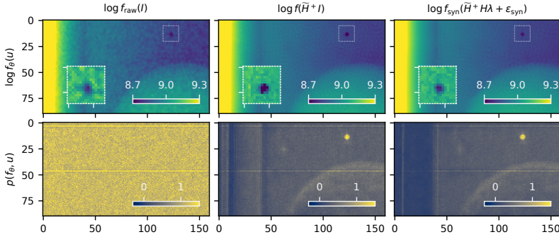
Figure 5.4: Blind-spot-denoised radiographs (figure 5.2), as well as their input-to-output correlation equation (5.15) summed over a 3-by-3 neighborhood (section 5.4.3). The left plots use unprocessed raw data, the middle plots deconvolved data, and the right plots synthetic independent noise. The granular background in the cylinder is a physical phenomenon due to stacking of particles. The output of f_{\text{raw}} displays checkerboard artifacts (inset in top left plot).
