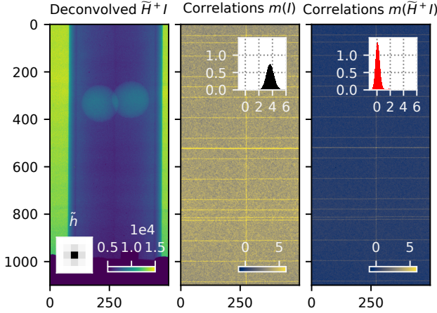
Figure 5.2: Deconvolution of 1,000 radiographs of a static PMMA cylinder containing two polystyrene balls, metal equipment, and non-uniform background radiation (cropped view, section 5.4.2). Left displays one radiograph and the kernel \tilde{h} . The middle and right show the correlation maps of I and \tilde{H}^+I . The lines of high correlation are due to inpainting of defective pixels during preprocessing. The probability density histograms show shifting and narrowing of the correlation distribution (black→red).
