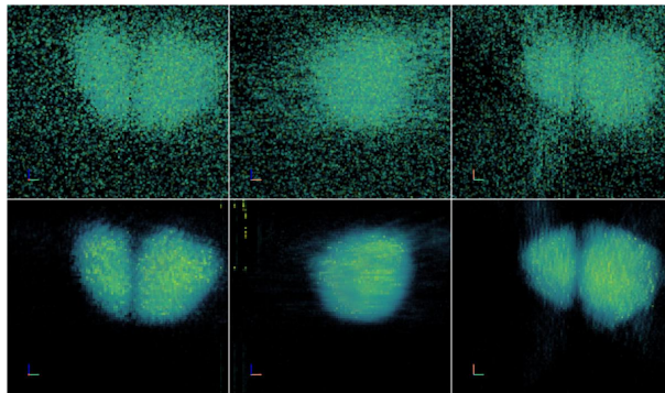
Figure 5.8: Ultra-sparse SIRT reconstructions of the noisy and denoised projections displayed in figure 5.7. Left: Side view along the projection axis of detector 1. Middle: Side view along the horizontal axis that is orthogonal to the projection axis. Right: Top view.
