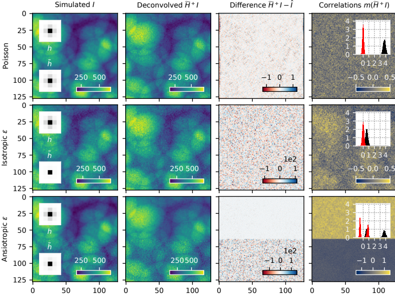
Figure 5.1: Kernel estimation and deconvolution evaluation: Simulated projection data of spheres impacted by high-noise (section 5.4.1). The top row contains pure Poisson noise. The middle row adds isotropic Gaussian noise with \sigma^2 = 400 . The bottom row only adds the Gaussian noise in the lower half-plane. The insets on the residual correlation maps (right column, see equation (5.13)) show histograms of the summed correlation over the whole image before (black) and after (red) deconvolution.
