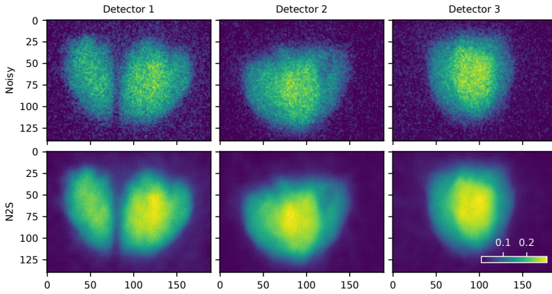
Figure 5.7: Top row: preprocessed projections (Chapter 2) of the single-bubble-injection experiment at timeframe 238/4500 (view is restricted to the bubble). Detector 1 shows that the bubble has split in two. Bottom row: Noise2Self network outputs.
