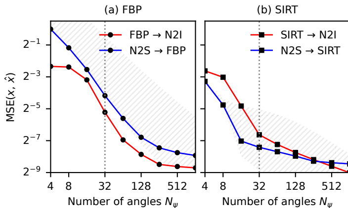
Figure 5.5: N2S and N2I combined with N_\psi sparse-view FBP and SIRT reconstructions (section 5.5.1) of the spherical phantoms [167], see figure 5.6 for a plot at the vertical indication line. Each data point is an individually trained U-Net [38] on N_\psi angles that is optimally stopped using ground truths. The limits of the shaded areas mark reconstruction from clean and noisy data.
