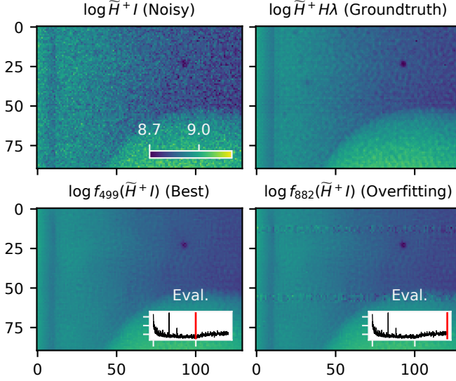
Figure 5.3: Training Noise2Self on the deconvolved data. Top row: Noisy and ground truth deconvolved radiographs (zoom into the upper-left part of figure 5.2). Bottom row: the trained Noise2Self U-Net evaluated on a single noisy image at an optimal point (epoch 499) and overfitting stage (epoch 882) during network training. Eval. plots the MSE evaluation of the trained network f_i at epoch i with the ground truth.
