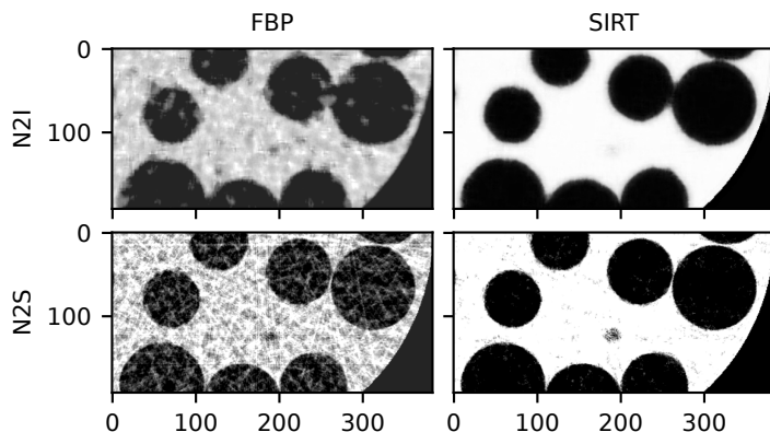
Figure 5.6: 192-by-384 region of interest taken from the N_\psi = 32 simulated reconstructions (see figure 5.5) at the central volume slice of the binary phantoms [167]. See figure 5.1 for an impression of the projections. A circular mask is applied to reduce the contribution of artifacts outside of the object in the MSE score of figure 5.5.
