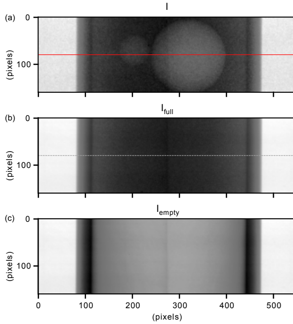
Figure 2.3: Raw measurements in a 550 \times 160 pixel detector region, showing (a) two spherical phantoms (diameters equal to 10 mm and 23 mm), (b) a full column reference (not fluidized), and (c) an empty column. The red and dashed rows are used to display noise statistics in Fig. 2.11.
