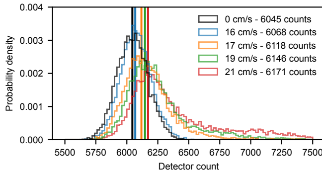
Figure 2.4: Detector count statistics for 1000-1200 measurements of a central pixel, for different superficial gas velocities of a fluidized bed. Vertical lines indicate the modes.
