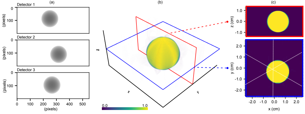
Figure 2.5: Reconstruction of a simulated sphere with a diameter D = 20 mm and a bubble fraction b = 1.0 . The visualization format is explained in Section 2.4.3.
