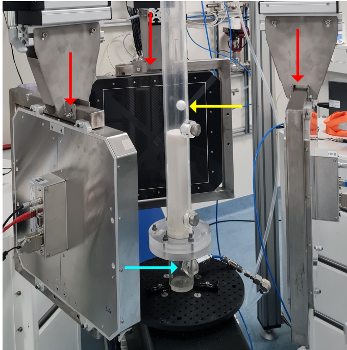
Figure 2.2: Photograph of the X-ray set-up with filled PMMA cylinder. Red arrows point to detectors, the yellow arrow to a polystyrene phantom (Section 2.5.2), and the blue arrow to the gas inlet. Sources are not in view.
