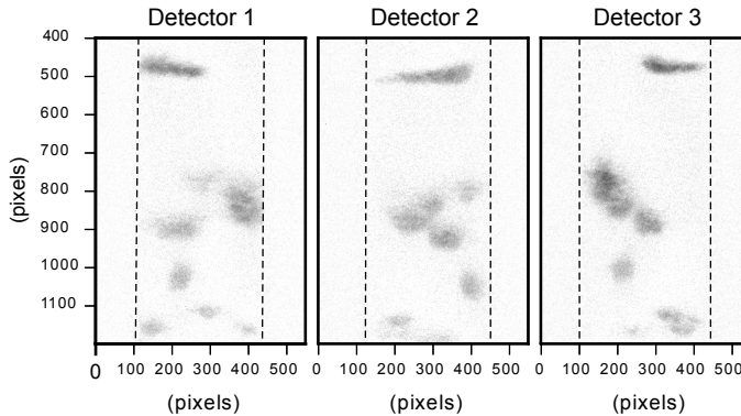
Figure 2.14: Projections y of timeframe 485 of the bed fluidized with a superficial gas velocity of 17 cm/s. The projections have been cropped to a region of interest, showing rows 400-1200. The column walls are indicated with dashed lines.
