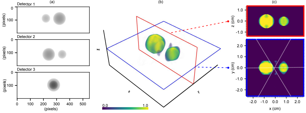
Figure 2.7: Reconstruction of two simulated bubbles with diameters D_1 \approx 1.23 cm and D_2 \approx 0.83 cm (74 and 50 voxels, respectively), for which the projections overlap on Detector 3. The visualization format is explained in Section 2.4.3.
