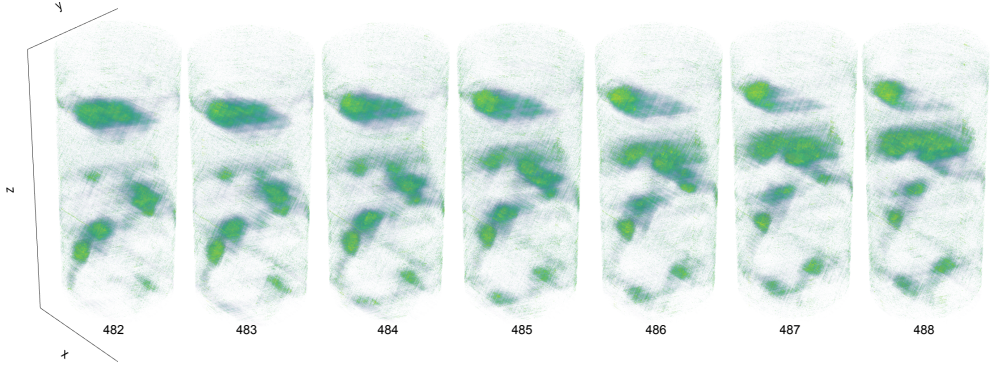
Figure 2.15: Timeframes 482-488 of the bubbling fluidized bed using an superficial gas velocity of 17 cm/s. For this visualization we enhanced the images by postprocessing with a low-weight ( \lambda = 1/0.065 ) total variation filter.
