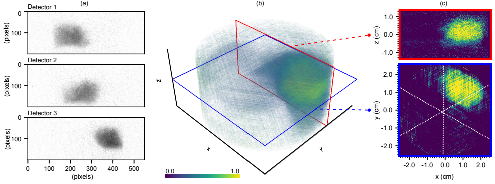
Figure 2.12: A solitary bubble that is extracted from frame 475 of the Geldart B fluidized bed reconstruction with a superficial gas velocity of 17 cm/s. The visualization format is explained in Section 2.4.3.
