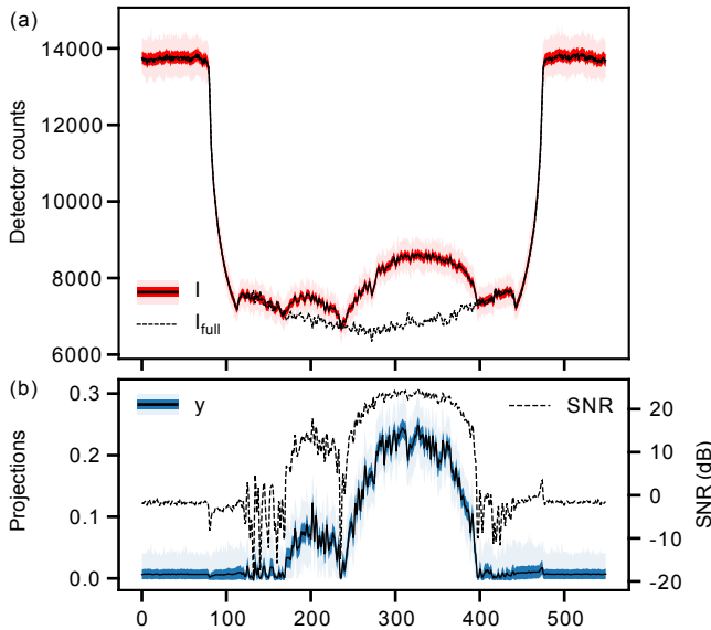
Figure 2.11: Panel (a) shows the line profile of raw measurement data of the marked detector row in panel (a) and (b) of Fig. 2.3. The computed noise statistics are shown in red (std.dev. in strong red, min/max values in light red). Panel (b) shows the same detector row, now after preprocessing, see the marked row in panel (a) of Fig. 2.9. Noise statistics of y are in blue.
