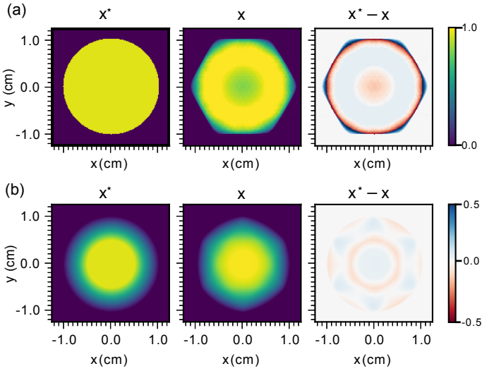
Figure 2.6: Reconstruction x of a spherical bubble x^* with b = 0.95 and diameter D = 20 mm. The bubble in panel (b) has a smoothed interface and is less affected by reconstruction artifacts.
