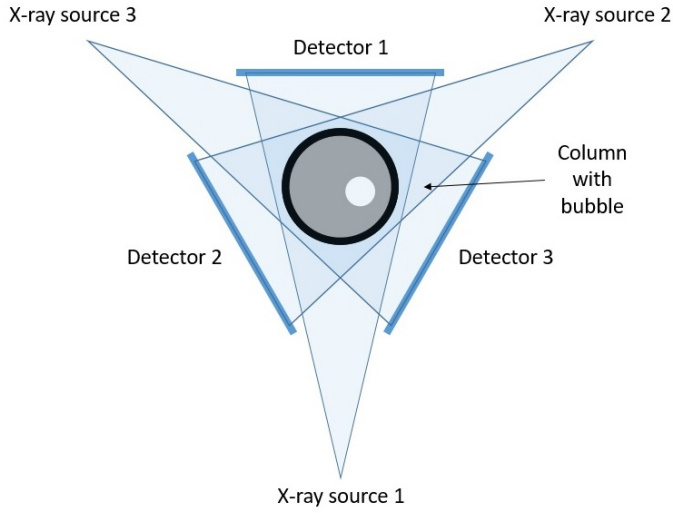
Figure 2.1: Top view schematic of the X-ray set-up (not to scale).
