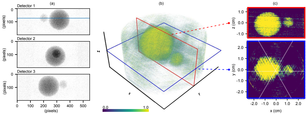
Figure 2.9: Reconstruction of two polystyrene phantoms, with diameters D_1 = 23 mm and D_2 = 10 mm, that overlap on the second detector. The reconstruction, panel (b), has been rotated to match Fig. 2.7. The detector row marked in blue is used to compute noise statistics in Fig. 2.11. The visualization format is explained in Section 2.4.3.
