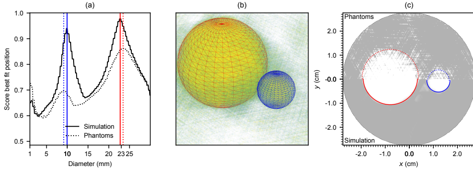
Figure 2.13: Template-matching of spheres with varying location and diameters to 10 mm (blue) and 23 mm (red) diameter bubbles, in a phantom experiment (dotted line) and a noiseless simulation (solid line). Panel (a) shows the best matching-score, Eq. (2.8), obtained for each diameter, panel (b) a 3D plot of best-matching templates overlaid onto the reconstruction of the phantoms (see Fig. 2.9), and panel (c) a horizontal cross-section of the reconstructions of noiseless simulations (bottom part) and phantoms (upper part) in grayscale coloring, onto which the boundaries of the best-matching spheres have been drawn.
