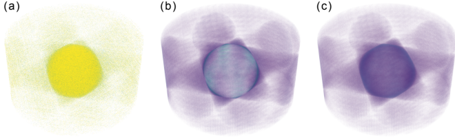
Figure 2.8: Reconstruction (a), bias (b) and variance (c), from a simulated spherical bubble, with a diameter D = 10 mm and a bubble fraction b = 1.0 . Zero-mean Gaussian noise with a variance of \sigma^2 = 2.6 \cdot 10^{-2} has been added to the projections. (b) and (c) are computed using 100 samples.
