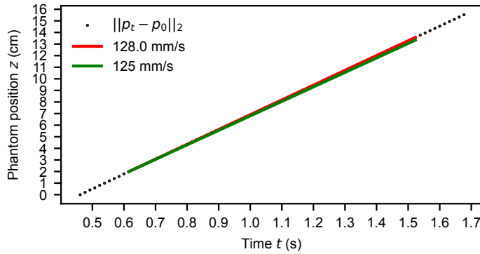
Figure 2.10: Least-square interpolation of positions p_t , obtained after presetting the traverse to 125 mm/s, and the detectors to 65 Hz.
