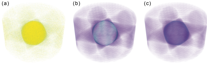
Figure 2.8: Reconstruction (a), bias (b) and variance (c), from a simulated spherical bubble, with a diameter D = 10 mm and a bubble fraction b = 1.0 . Zero-mean Gaussian noise with a variance of \sigma^2 = 2.6 \cdot 10^{-2} has been added to the projections. (b) and (c) are computed using 100 samples.
