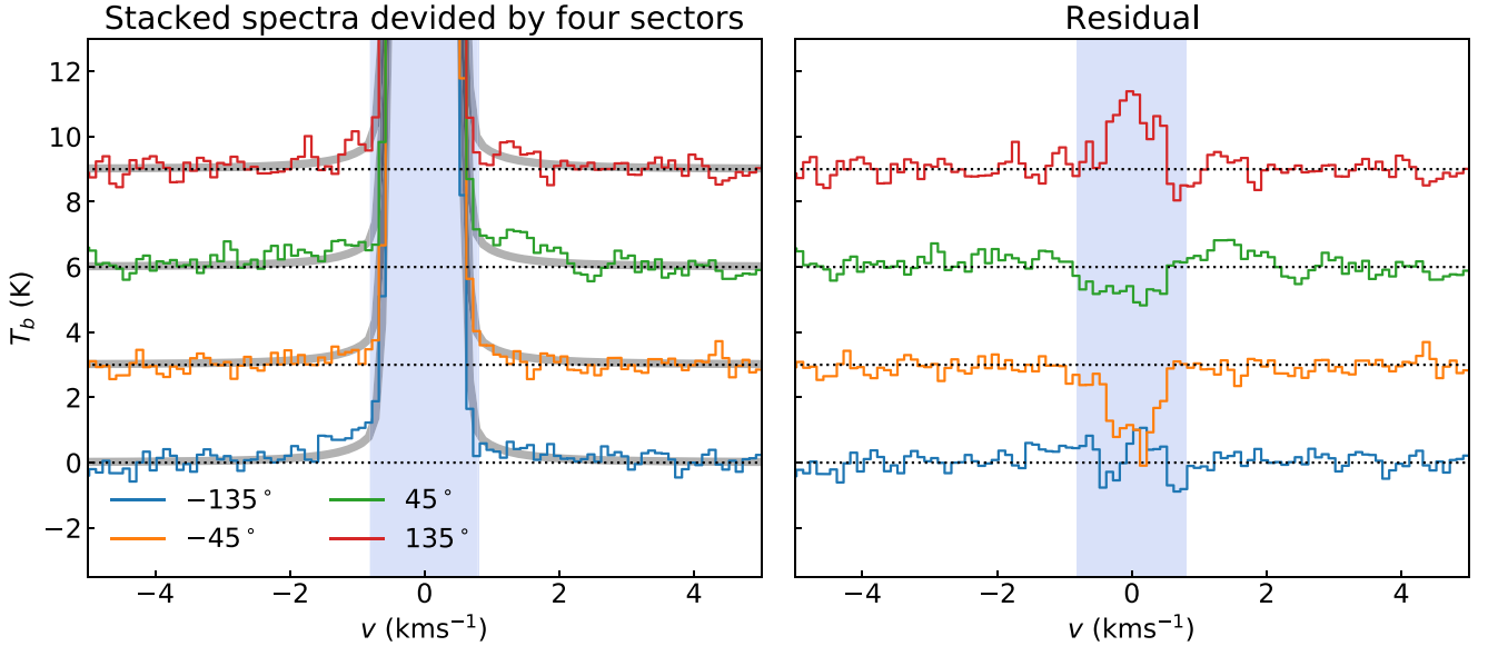
Figure 10. (Left) Radially averaged azimuthally stacked spectra at r = 0.4 - 0.8 . The stacked azimuthal range is limited to one-quarter of an annulus, and the center azimuthal angle is shown in the legend. The gray solid lines indicate the fiducial model spectrum. (Right) Residual of observed spectra after subtracting the fiducial model. Note that the spectra are vertically shifted for visibility purposes. The blue-shaded area indicates the optically thick line cores.
