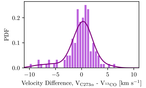
Figure 10. The velocity difference between each \text{C}273\alpha component and the ^{13}\text{CO} component nearest in velocity for a given aperture. The standard deviation of this distribution is 2.9 \text{ km s}^{-1} .
