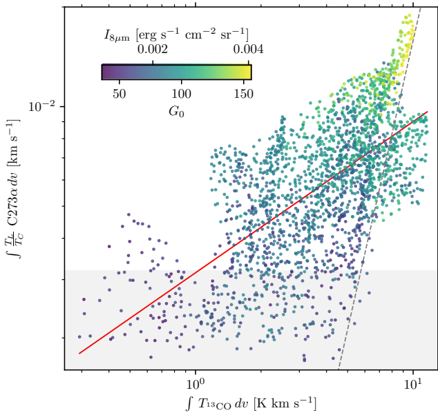
Figure 8. A comparison of the point-by-point velocity-integrated ^{13}\text{CO} and \text{C}273\alpha emissions. The gray shaded region indicates where \text{C}273\alpha has 3 \leq \text{S/N} < 5 . We note that all ^{13}\text{CO} points have an \text{S/N} > 5 . The data points are colored by I_{8\mu\text{m}} and the corresponding estimate of G_0 (see Section 7). The red solid line shows the best-fit power law with slope a = 0.46 , while the gray dashed line has a power-law slope of a = 2.9 and has been included for illustrative purposes to indicate the possible “high-intensity regime”.
