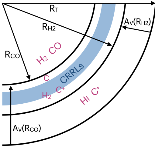
Figure 13. Illustration of a model cloud showing the parameters defined in the M. G. Wolfire et al. (2010) framework. R_{CO} is the radius of the CO core. R_{H_2} is the radius where 2n_{H_2} = n_{H\,I} with equal mass density in H atoms and H_2 molecules. R_T is the total cloud radius. Within R < R_{CO} , gas is mainly CO and H_2 . Within the range R_{CO} < R < R_{H_2} , gas is mainly H_2 , whereas the gas-phase carbon is mainly C and C^+ . The CRRLs arise from a C^+ layer that is mainly H_2 . Within R_{H_2} < R < R_T gas is mainly H I and gas-phase carbon is mainly C^+ . A_V(R_{H_2}) is the magnitude of extinction measured from the outer radius to R_{H_2} , and A_V(R_{CO}) is the magnitude of extinction measured from the outer radius to R_{CO} .
