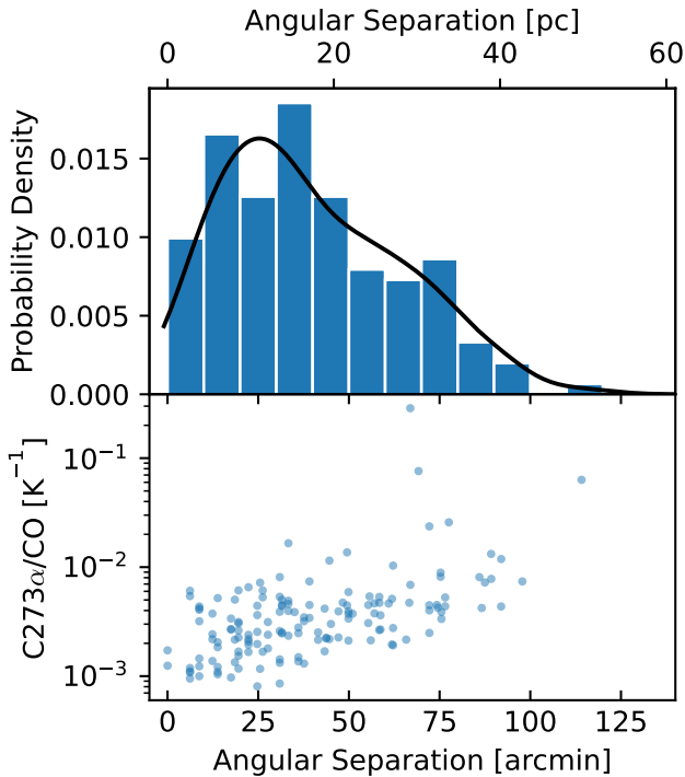
Figure 9. Top: spatial separation between \text{C}273\alpha peaks and the closest ^{13}\text{CO} peak identified in channel maps. A maximum in the distribution is found at 26' (12 pc), which is larger than the pointing accuracy of 1' . Bottom: the angular separation plotted against the \text{C}273\alpha/^{13}\text{CO} intensity ratio at the pixel of the \text{C}273\alpha peak. The intensity ratio of \text{C}273\alpha/^{13}\text{CO} tends to be larger when the angular separation between intensity peaks is larger.
