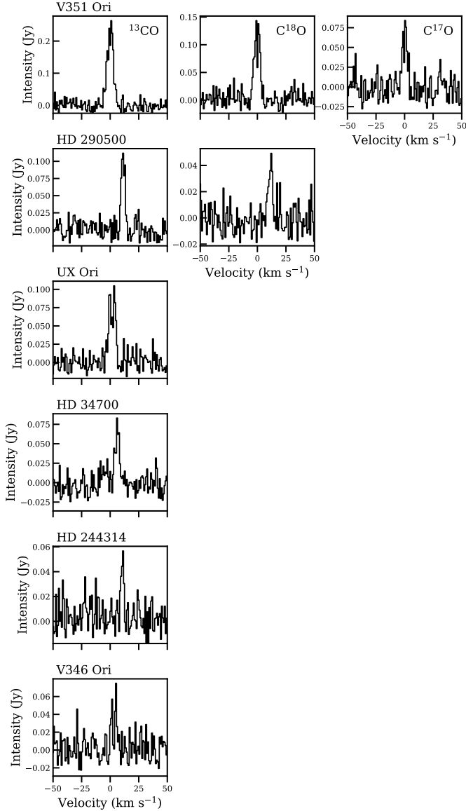
Fig. 3. Spectra of the disks in which 13 CO, C 18 O, or C 17 O are detected. The spectra are centered on the frequencies of the emission lines and are binned to 1 km s -1 .
