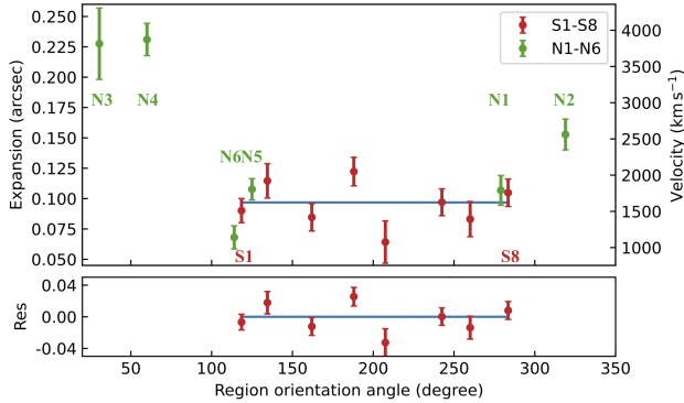
Figure 7. As in Figure 6, but for the final expansion estimates. The expansion of each region (“corrected shifts” in Table 5) is based on the raw shifts shown in Figure 6, corrected for the PSF bias and COE bias. The blue solid line shows the average expansion of the S1–S8 regions.
