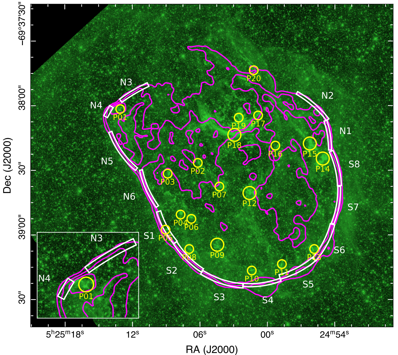
Figure 10. M. A. Dopita et al. (2018) shocked H\alpha -cloud regions displayed on the HST H\alpha (F658N) image with Chandra 2019–2020 (1.2–7.0 keV) contours in purple. Our expansion and spectral analysis regions are plotted in white. The inset shows an expanded view of the northeast. Cloud P01 shows indications of having interacted with the blast wave in the northeast—see the indentation in the X-ray contours in the inset and the X-ray enhancement in Figure 1. The small cloud P05 shows no indication of significant interaction in region S1.
