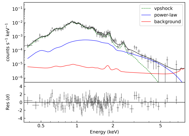
Figure 11. The spectrum of shock region N4 fit with a vpshock + power-law model and the background model. The black points and line are the spectral data and model, respectively. The green dashed line is the vpshock component. The blue line is the power-law component with an index of three. The red line is the background model.
