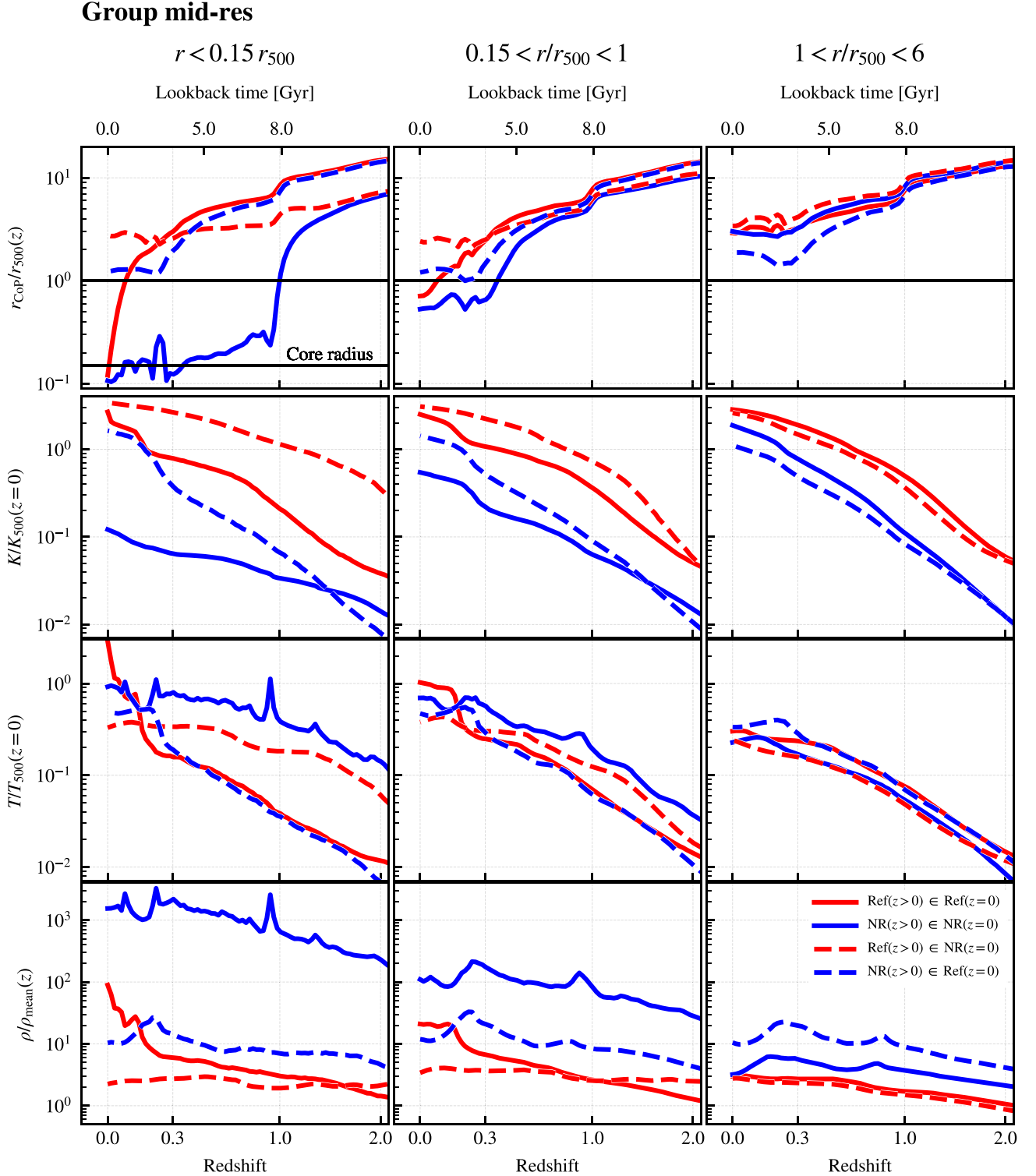
Figure 6. From top to bottom: Lagrangian history of the median scaled halocentric distance ( r_{\text{CoP}} ), entropy ( K ), temperature ( T ), and density ( \rho ) of gas particles in the group at mid-res. From left to right: the particles are identified in three spherical regions defined at z=0 : the core ( r < 0.15 r_{500} , left), the rest of the intragroup medium ( 0.15 < r/r_{500} < 1 , centre), and outside r_{500} (right), as indicated at the top of the panels. These radii are also indicated in the overview maps of Fig. 2. The particles in each spherical region are selected in three ways: (i) gas particles in Ref that end up hot and inside the region in Ref at z=0 (red solid); (ii) gas particles in NR that end up inside the region in NR at z=0 (solid blue); (iii) gas particles in NR that end up in the region in Ref at z=0 (dashed blue); and (iv) gas particles in Ref that end up in the region in NR at z=0 (dashed red). The entropy and temperatures are normalized to the self-similar value at z=0 ; the density is normalized to the mean matter density at each redshift, \rho_{\text{mean}}(z) = \Omega_m \rho_{\text{crit}}(z) ; the radius is normalized to r_{500}(z) and computed at each redshift. The horizontal black lines indicate r_{500} and the core radius, 0.15 r_{500} .
