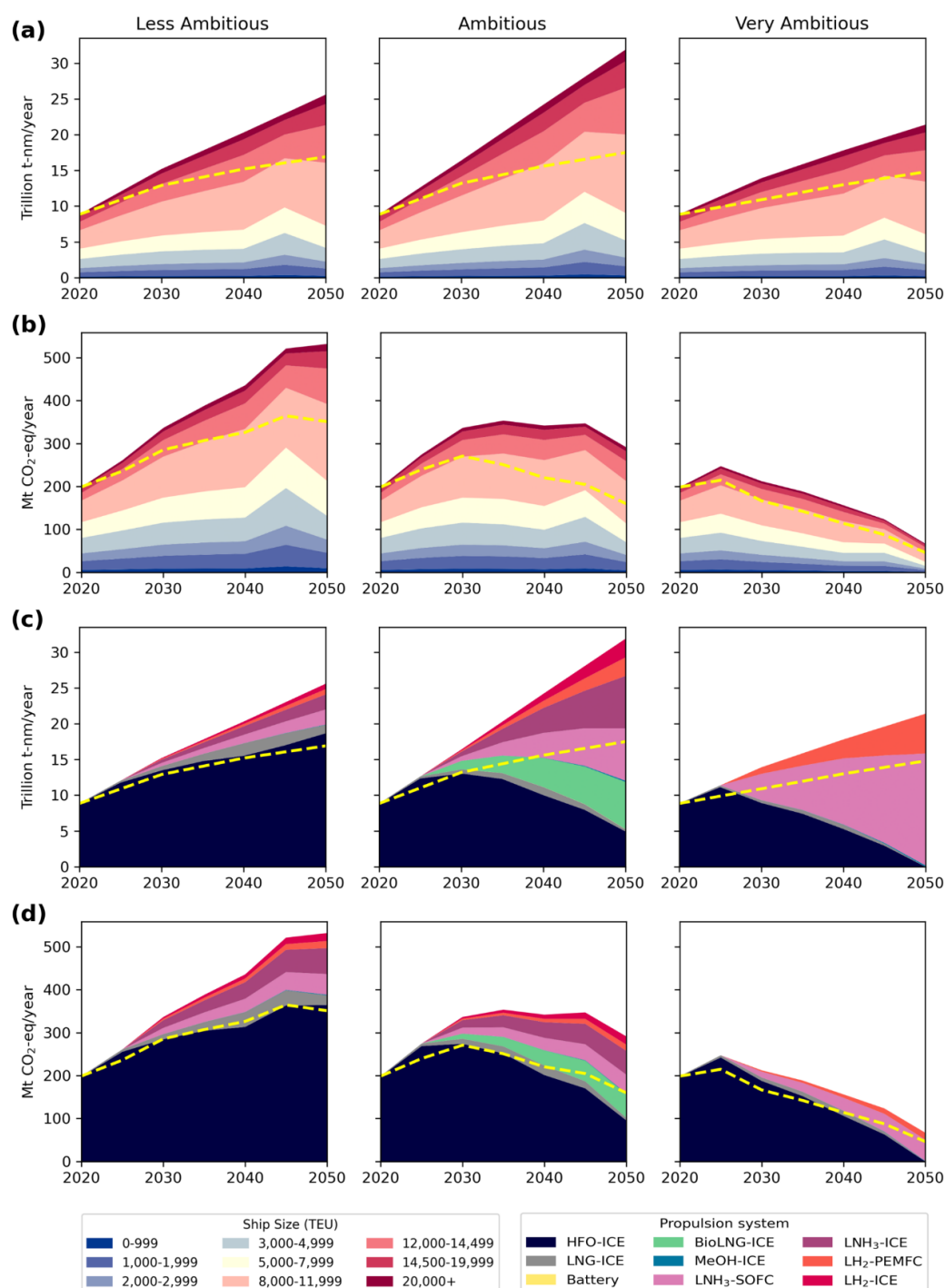
Figure 5.4. Annual global container shipping transport demand and GHG emissions by ship size (a, b) and propulsion systems (c, d). In this figure, the stacked values are based on predictions from the logistic model. The yellow dashed lines represent the total annual transport demand and GHG emissions estimated by the gravity model for comparison.
