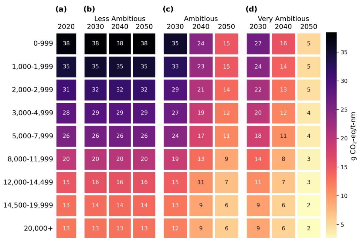
Figure 5.5. Weighted average GHG emissions of ship fleet by sizes (TEU). In the figure, (a) represents the value in 2020, (b), (c) and (d) presents the values for 2030, 2040 and 2050 in the Less Ambitious, Ambitious and Very Ambitious scenarios, respectively.
