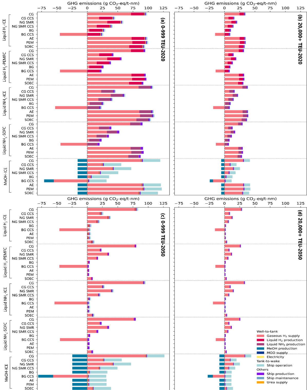
Figure 5.3. Prospective GHG emissions from H 2 -based propulsion systems for container ships in 2020 and 2050 by H 2 source in the Ambitious scenario. In this figure, CG=coal gasification, NG SMR=steam methane reforming of natural gas, BG=biomass gasification, CCS=carbon capture and storage AE=alkaline electrolyzer, PEM=proton exchange membrane electrolyzer, and SOEC=solid oxide electrolysis cell. Gaseous H 2 production via biomass gasification with carbon capture and storage, and CO 2 capture through direct air capture can contribute to negative emissions. Prospective GHG emissions from H 2 -based ships by H 2 source under the Less Ambitious scenario are shown in Figure S4.7 of the SI. In the Very Ambitious scenario, the H 2 market consists exclusively of 100% renewable electrolytic H 2 from PEM using newly built onshore wind power, without contributions from other technologies. Prospective GHG emissions from H 2 -based ships by H 2 source under the Very Ambitious scenario are the same as those shown in Figure 5.2. To convey the information effectively, only the results for the smallest and largest ship categories in 2020 and 2050 are shown, as the outcomes for other ship categories and years fall within these ranges.
