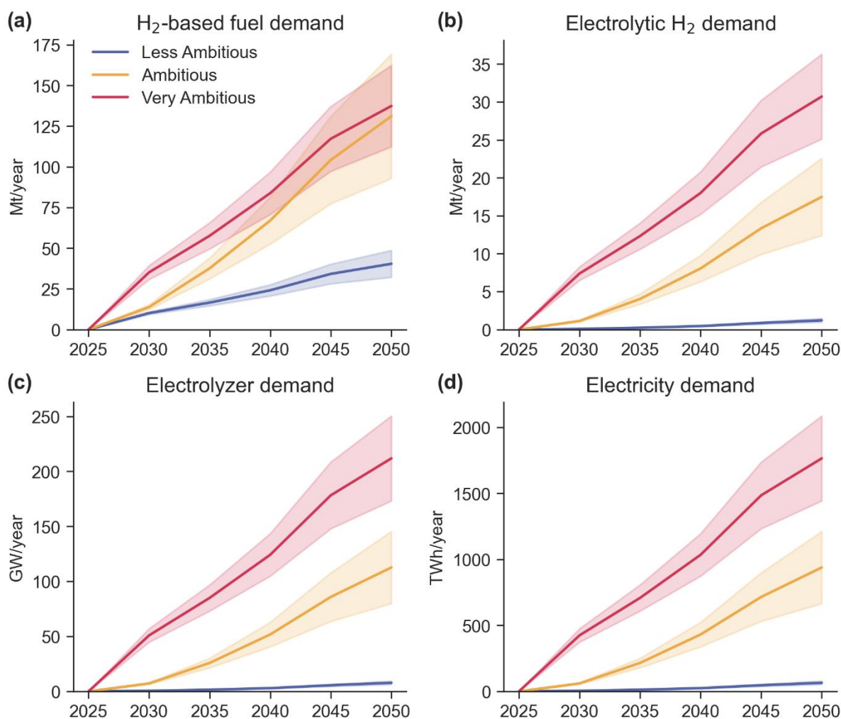
Figure 5.7. Demand for (a) H_2 -based fuels, (b) electrolytic gaseous H_2 , (c) electrolyzer capacity, and (d) electricity required for electrolytic H_2 production in global container shipping under the Less Ambitious, Ambitious, and Very Ambitious scenarios. In this figure, the higher and lower boundaries represent the values corresponding to the transport demand estimated by the logistic and gravity models, respectively; while the line is the average value.
