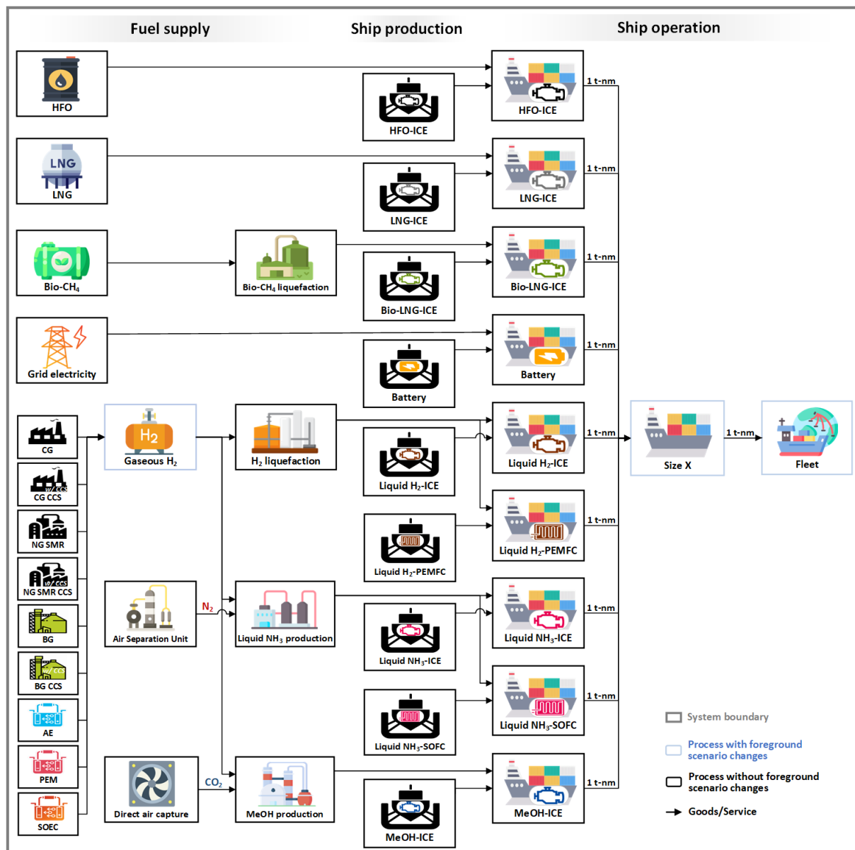
Figure 5.1. The LCA model of container shipping. In this figure, CG=coal gasification, NG SMR=steam methane reforming of natural gas, BG=biomass gasification, CCS=carbon capture and storage AE=alkaline electrolyzers, PEM=proton exchange membrane electrolyzers, SOEC=solid oxide electrolysis cells, ICE=internal combustion engines, PEMFC=proton-exchange membrane fuel cells, SOFC= solid oxide fuel cells, HFO=heavy fuel oil, LNG=liquefied natural gas, and bio-LNG=liquefied biomethane. Nine ship size categories are considered. For LNG-ICE, bio-LNG-ICE, liquid H 2 -ICE, liquid NH 3 -ICE and MeOH-ICE, a small amount of marine gas oil is required as pilot fuel. Size x represents nine container ship categories with capacities ranging from 0–999 TEU, 1,000–1,999 TEU, 2,000–2,999 TEU, 3,000–4,999 TEU, 5,000–7,999 TEU, 12,000–14,499, 14,500–19,999, and 20,000+ TEU. TEU (twenty-foot equivalent unit) refers to a standard 20-foot-long shipping container. Battery-powered ships are only applicable to the 0–999 TEU category.
