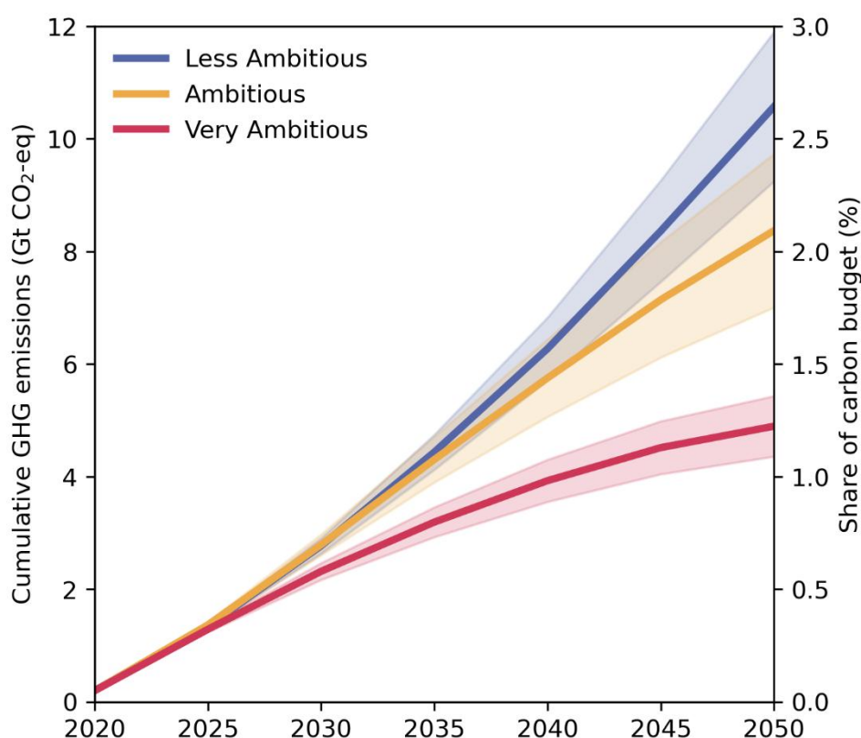
Figure 5.6. Cumulative GHG emissions of global container shipping between 2020 and 2050 under the Less Ambitious, Ambitious and Very Ambitious scenarios, and their share of the carbon budget for the 1.5 °C target. In this figure, the upper and lower boundaries of the range represent the values from the logistic and gravity models, respectively, while the line indicates the average value.
