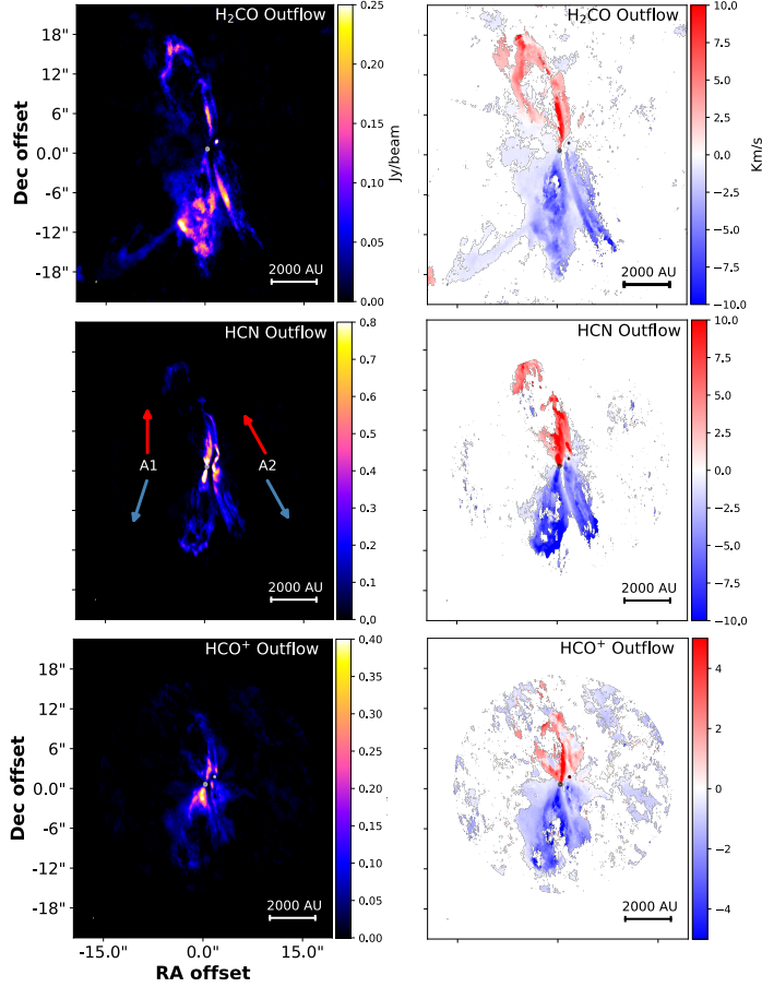
Figure 3.2: Integrated emission and velocity maps of the three main outflow tracers in our spectra: \text{HCN} , \text{H}_2\text{CO} , and \text{HCO}^+ generated using the short baseline line data for IRAS4A. The emission from the outflows of both sources, IRAS4A1 and IRAS4A2, is resolved and can be distinguished separately. In the figures, the dust continuum emission of IRAS4A1 and IRAS4A2 is outlined in small white contours, showing 5\sigma and 10\sigma . The beam is drawn in the lower left part of each panel, 0.28'' \times 0.17'' for \text{HCN} and \text{HCO}^+ and 0.44'' \times 0.28'' for \text{H}_2\text{CO} . The red and blue arrows in the middle-left panel indicate the outflow directions of IRAS4A1 (left) and IRAS4A2 (right) (Chahine et al. 2024), respectively.
