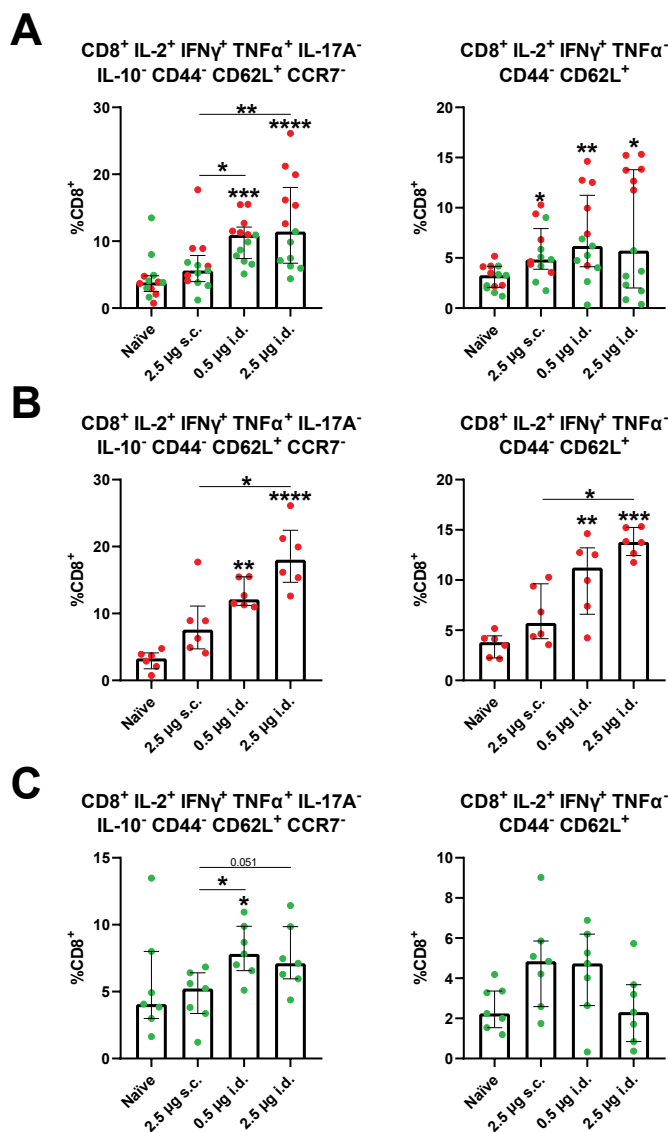
Figure 5. Variations in the abundance of CD8 + T-cell populations within restimulated splenocytes from immunized mice. Each graph identifies the markers characterizing the respective populations and displays the percentage values of these populations as median \pm IQR within the CD3 + CD19 - CD4 - CD8 + cell subset. A) Combined results from both experiments. Each dot represents a single mouse, and the results of the same experiment are shown in one color. n = 13 (mice). B) Results from the first experiment. n = 6 (mice). C) Results from the second experiment. n = 7 (mice). The minimal number of events used in the analysis was 20,000. Groups represent: naïve – unimmunized mice, 2.5 \mu\text{g} s.c. – immunization with 2.5 \mu\text{g} AER subcutaneously, 0.5 \mu\text{g} i.d. – immunization with 0.5 \mu\text{g} AER intradermally, 2.5 \mu\text{g} i.d. – immunization with 2.5 \mu\text{g} AER intradermally.
