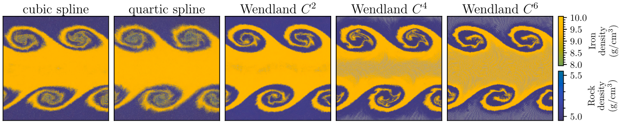
Fig. D.24. The effect of kernel choice in REMIX KHI simulations between Earth-like iron & rock. Plotted at time t = 2 \tau_{KH} , for 5 different kernel functions. Particles are coloured by their material type and density. These simulations have a resolution of N_i = 128 , as described in §4.3.2.
