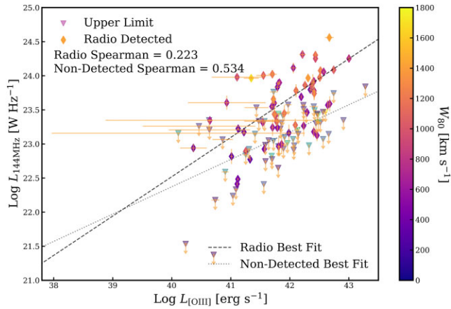
Figure 8. L_{144\text{MHz}} as a function of total L_{[\text{OIII}]} with the W_{80} traced by a colour scale. Radio detected AGN are plotted with diamonds and the upper limits for the radio non-detected AGN are shown by the downward triangles. The dashed black line show the best fit relationship for the radio detected AGN and the grey dotted line shows the best fit to the upper limits of the radio non-detected population.
