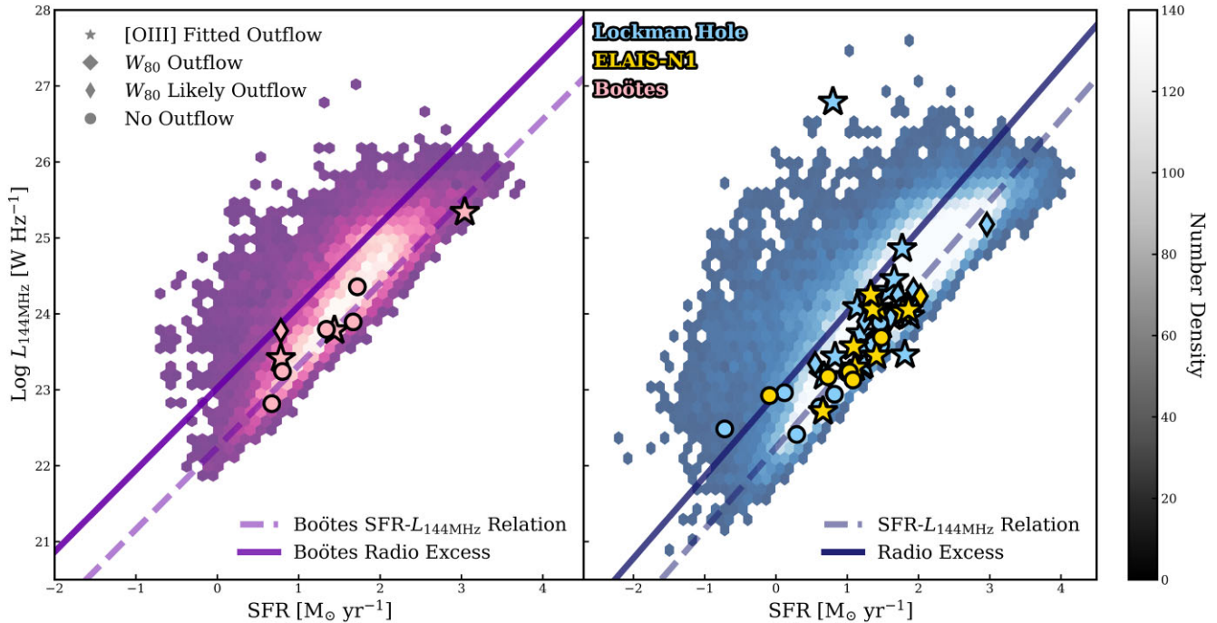
Figure 9. The relationship between SFR and L_{144\text{MHz}} . The left subplot shows the result of the Boötes field (pink markers) and on the right Lockman Hole (blue markers) and ELAIS-N1 (yellow markers), the fields have been split because of the need for an extra adjustment to the radio excess in Boötes. Error bars are included but are too minimal to see. No upper limits are shown for the radio non-detected AGN because we do not have access for reliable SFR measurements for these AGN. The background hexagon bins show the distribution of sources with reliable SFR measurements with Boötes in purple and Lockman Hole and ELAIS-N1 combined in blue, where a hexagon is plotted for areas where there is four or more sources. On each panel, the faint dashed line shows the SFR– L_{144\text{MHz}} relation, which is the same for both fields. The solid line shows the radio excess divide which is 0.7 dex above the SFR– L_{144\text{MHz}} for Lockman Hole and ELAIS-N1 with a slight redshift adjustment for Boötes. The over laid points with black edges are the sources within the best matched populations. The stars are sources with an [O III] fitted outflow, thick diamond host an W_{80} outflow and thin diamonds are AGN with a likely outflow. Circles represent sources that show no indication of an outflow. The colour scale traces the number density of each hexagon and is shown as grey as the scale is the same for both subplots, hence it would be pink for Boötes and blue for Lockman Hole and ELAIS-N1.
