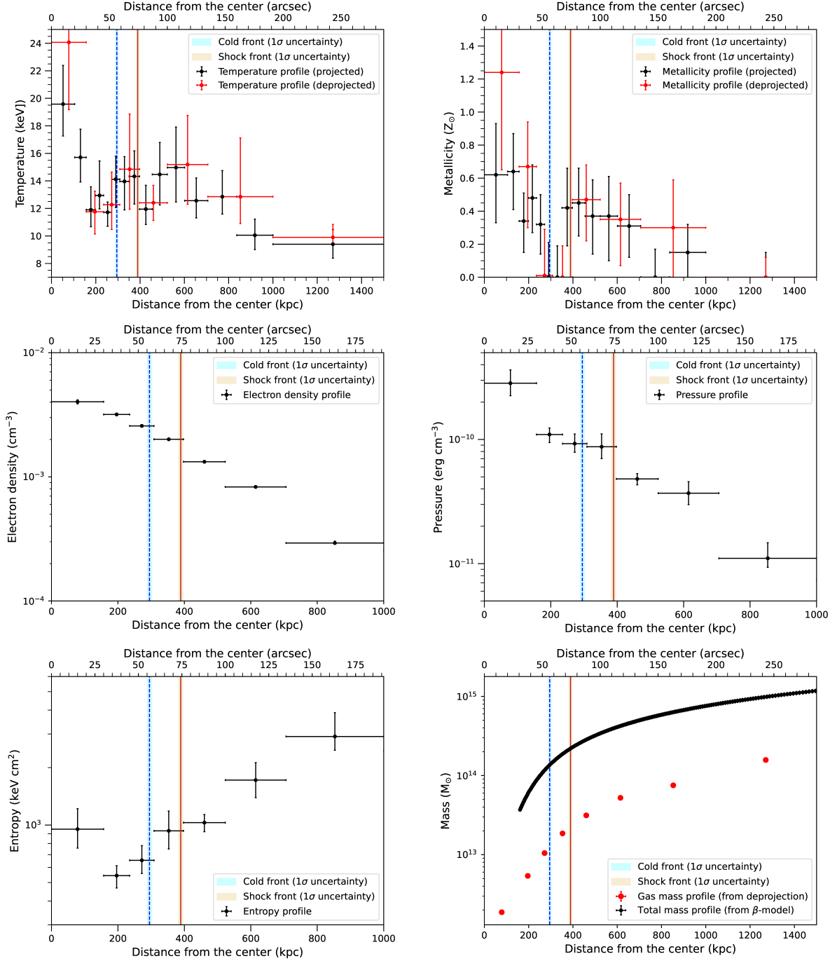
Fig. 6. Radial profiles of PLCKG287 obtained from the Chandra spectral analysis. Top panels: Temperature ( left ) and metallicity ( right ) from the projected (black) and deprojected (red) spectral analysis (see Tables 3 and 4). Middle and Bottom panels: Density ( middle left ), pressure ( middle right ), entropy ( bottom left ) and integrated gas mass ( bottom right , red points) from the deprojected spectral analysis (see Table 4). The total mass profile ( bottom right , black solid line) is estimated from the circular \beta -model by assuming an isothermal kT \sim 12.7 keV. In all panels, the vertical lines show the position of the fronts discussed in Section 4 (the dashed blue line and solid red line indicate the cold front and shock, respectively).
