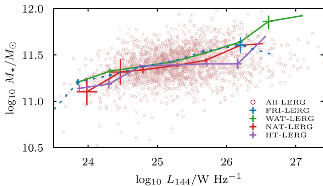
Figure 22. As in Fig. 17, but now showing the bent-tail LERG sources from our sample. The FRI plot is also included for reference, shown as dotted lines.
