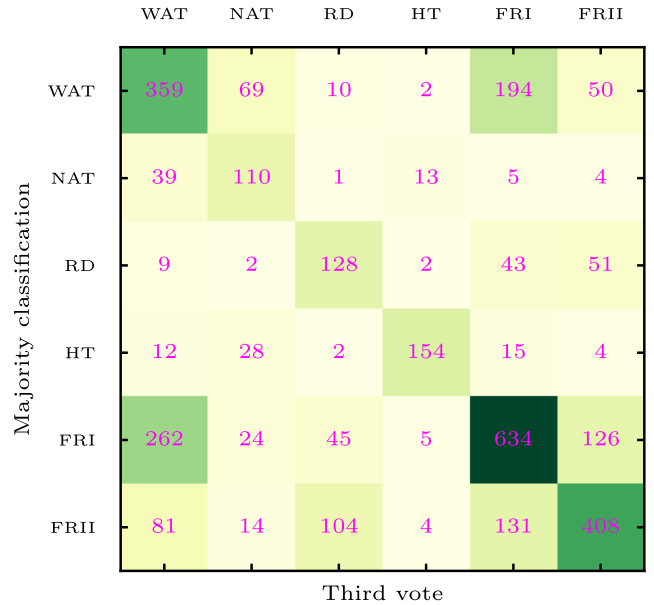
Figure 1. The heatmap shows a strong diagonal dominance, indicating that most objects received the same classification from two voters. The most significant densities are observed along the diagonal, which suggests consistency among the voters, whereas the off-diagonal cells represent cases where objects received mixed classifications, indicating ambiguity or transitional characteristics. For example some WATs were also voted as FRIs, and some relaxed sources were voted as FRIIs.
