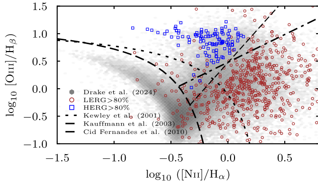
Figure 4. The BPT diagram highlighting the positions of objects in our sample, spectroscopically classified as HERG (squares) and LERG (circles) using the 80 per cent threshold, overlaid on the D24 sample (hexagons).
