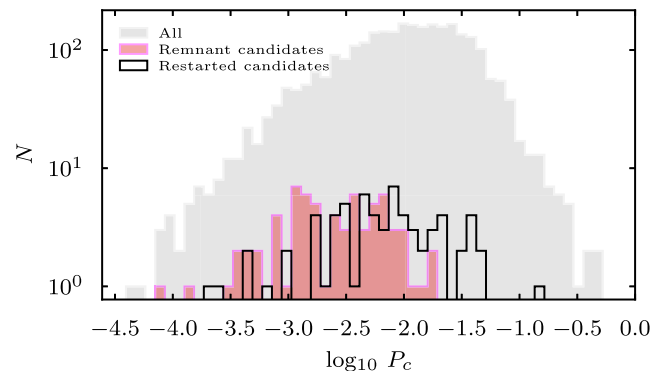
Figure 23. Core prominences for candidate remnant and restarted sources in our sample, with the general RLAGN population shown in the background.
