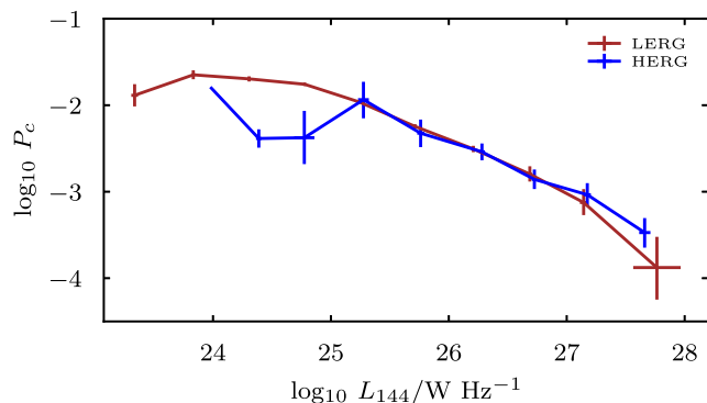
Figure 14. The distribution of core prominence as a function of radio luminosity. The points, binned by luminosity with a bin size of \Delta \log_{10} L_{144}/\text{W Hz}^{-1} = 0.5 , represent the mean values with bootstrapped errors, estimated from the 68th percentile confidence interval.
