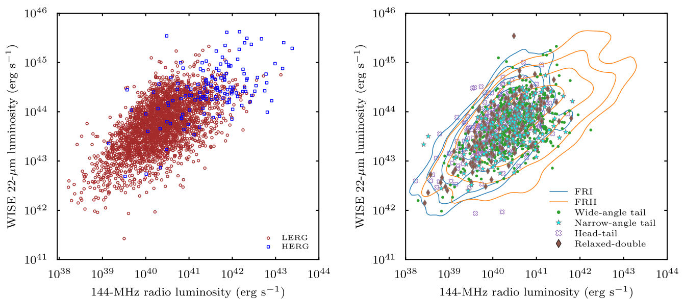
Figure 10. The figure shows the distribution of optical emission-line classifications (left panel) and morphological classifications (right panel) on the WISE W4 luminosity versus radio luminosity plane. Of the 2828 sources in our sample, only 766 have W4 detections, while the rest are represented as upper limits.
