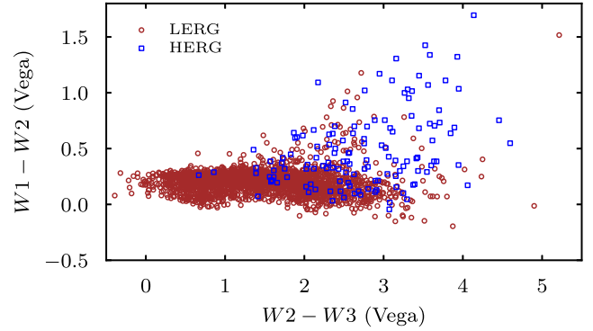
Figure 8. The position of HERGs and LERGs in WISE colour–colour plots. For a discussion of upper limits, refer to the caption in Fig. 9.
