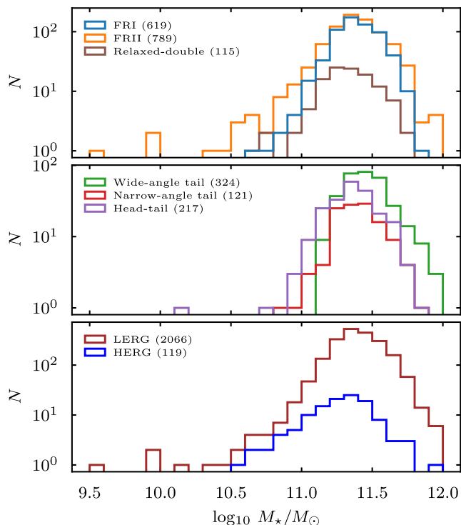
Figure 11. Distribution of host galaxy mass categorized by morphology (top and middle) and emission-line class (bottom). The legend provides a breakdown of each classification with reliable host mass estimates.
