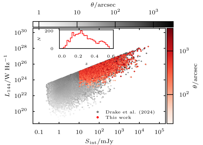
Figure 3. The distribution of our sample is shown in the radio luminosity versus total flux density plane overlaid on the broader D24 sample. The horizontal and vertical colour bars illustrate the angular size of the D24 sample and our sample, respectively.
