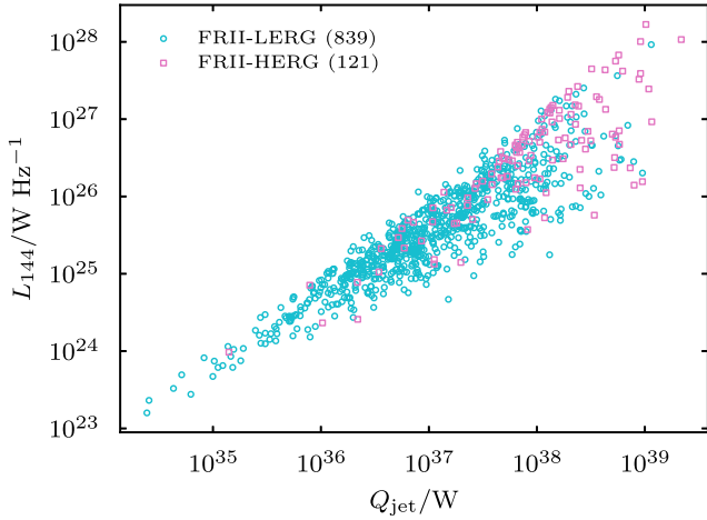
Figure 20. Distribution of the LERG and HERG populations in the FRII sample on the Q_{\text{jet}} - L_{144} plane, with jet powers estimated using the methods of Hardcastle et al. (2019).
