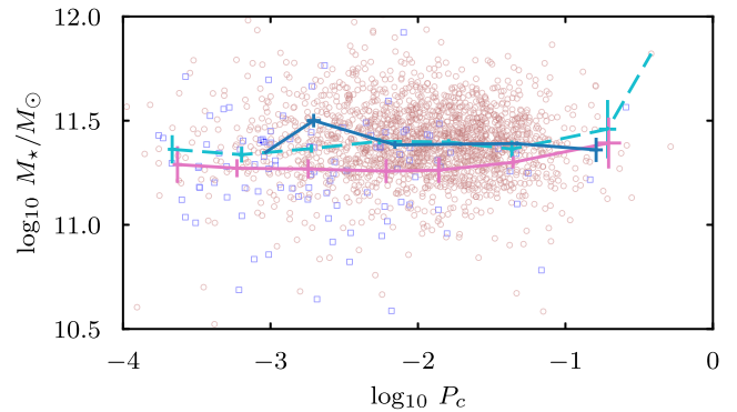
Figure 18. The dependence of core prominence on host galaxy mass for FRIs and FRIIs in the LERG/HERG sample. Error bars represent bootstrap estimates of bin mean values ( \Delta \log_{10} P_c = 0.5 ) with 68 per cent confidence intervals. Legend same as Fig. 17.
