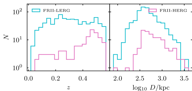
Figure 19. Comparison of HERG (pink) and LERG (cyan) distributions in redshift and physical size within the FRII sample. The number of sources in this plot is given in the legend of Fig. 20. Note that selection effects may influence the distribution of sources on these plots.
