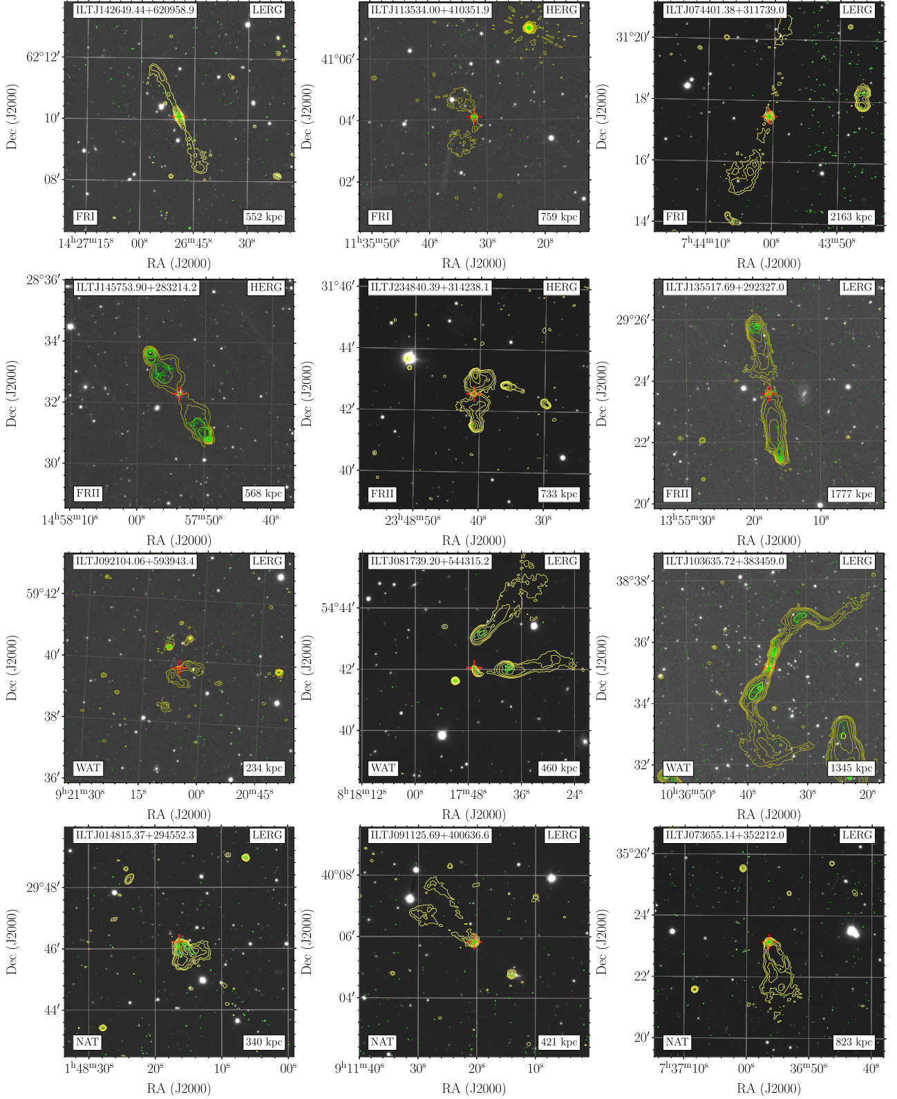
Figure A1. Representative images from our final morphological classifications are shown in this figure following visual inspection. LOFAR and VLA contours, in gold and green respectively, are overlaid on i -band Pan-STARRS images, with optical IDs marked by a plus sign. Physical size estimates are provided in the bottom right corner of each panel to highlight ‘normal’ and candidate giant radio galaxies. Continued in Fig. A2.
