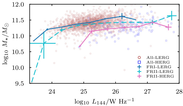
Figure 17. The dependence of radio luminosity on host galaxy mass, showing the distribution of FRI and FRII galaxies in the LERG/HERG sample. Errors and luminosity bin size as calculated in Fig. 14.
