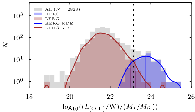
Figure 5. An adaptation of the D24 HERG/LERG classification criteria utilizing the specific [O III] emission-line luminosity for radio-excess AGN with available [O III] and stellar mass measurements. Objects with \log_{10} (L_{[\text{OIII}]} / M_{\star}) > 23.14 are classified as HERGs. Those below this threshold are classified as LERGs.
