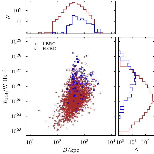
Figure 7. The distribution of LERGs (shown as brown open circles) and HERGs (blue open squares) in P–D space. This histograms highlight the coverage in size and luminosity for LERG and HERG in our sample.
