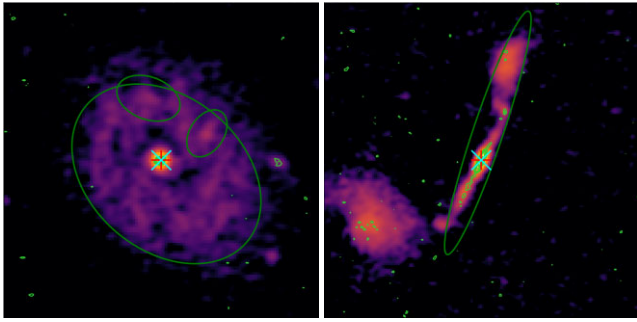
Figure 2. Example images used in the visual classification, showing VLASS contours (green) overlaid on the LOFAR image. The ellipses indicate source component identification by PYBDSF, the cyan cross marks the optical position, and the red plus sign denotes the centroid of the radio source. As noted in the caption of Fig. 1, the right image represents an object that received two votes for the FRI category, while the third vote was assigned to the WAT category. However, the two FRI votes, along with further inspection, were sufficient to classify it as an FRI in our final selection. The image on the left represents objects that were rejected due to SF signatures, as explained in the text.
