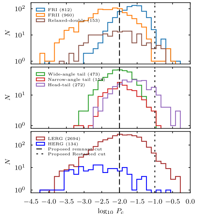
Figure 12. Core prominence ( P_c ) distribution for the various morphological classes (top and middle) and emission-line class (bottom) in our sample. Upper limits are also included on these plots. We additionally included proposed cuts used in the selection of remnant and restarted candidates (e.g. Brienza et al. 2017; Jurlin et al. 2021).
