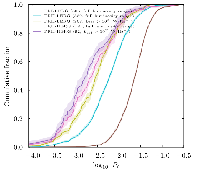
Figure 13. The distribution of core prominence within the FRII sample, separated into LERG and HERG. The analysis includes the full luminosity range and a subset of high luminosity FRIIs, as described in the text. The FRI LERG sample is included for comparison. The number of objects for each category is included in the legend. The shaded regions represent the 1\sigma errors, estimated using the bootstrapping procedure.
