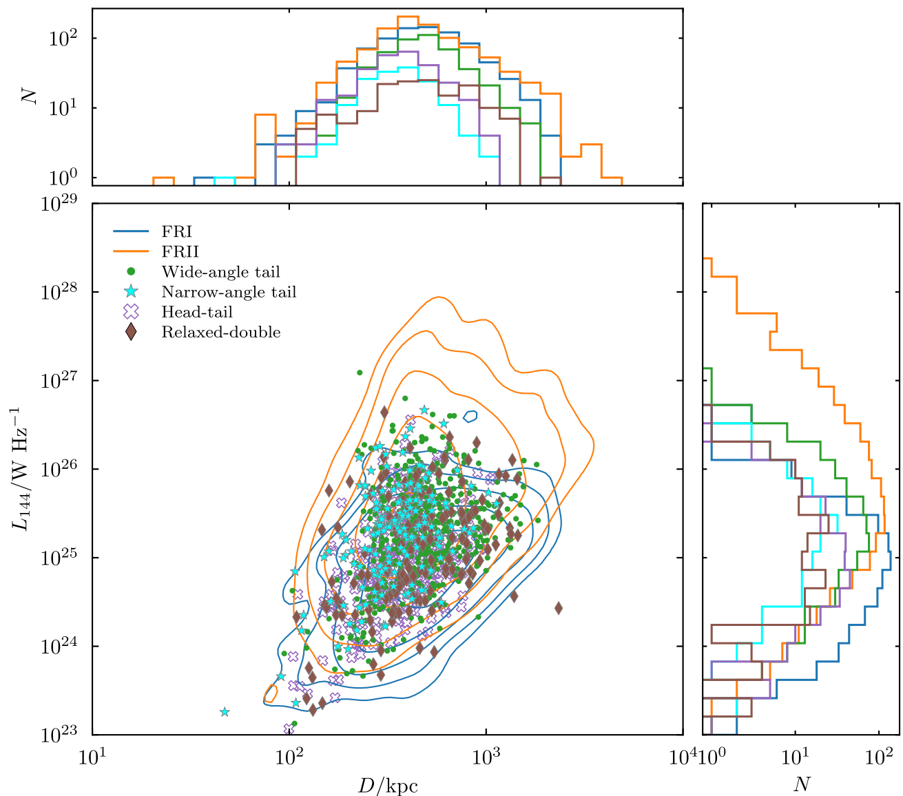
Figure 6. P–D diagram showing the distribution of visually classified morphological sources in our sample. Histograms for size and luminosity are included to highlight the range covered by each object.
