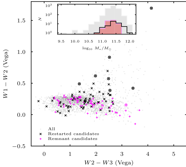
Figure 24. Mid-IR environments of remnant and restart candidates. The inset shows the distribution of host galaxy mass for these categories, overlaid on the general RLAGN population in our sample. Circles highlight, respectively, remnant and restart candidates spectroscopically classified as HERGs.
