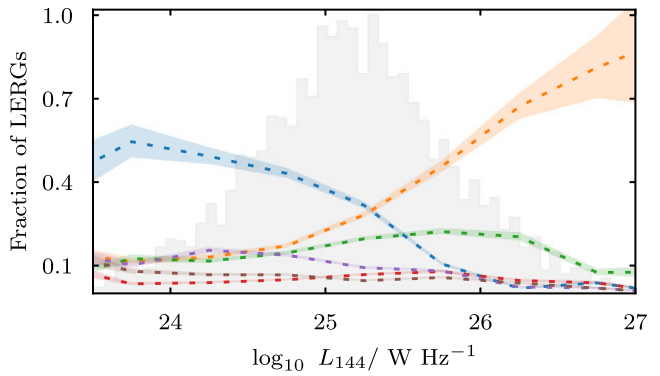
Figure 16. Fraction of morphological classes in the LERG sample as a function of redshift (left panel) and radio luminosity (right panel). Shaded regions are depicted as in Fig. 15.
