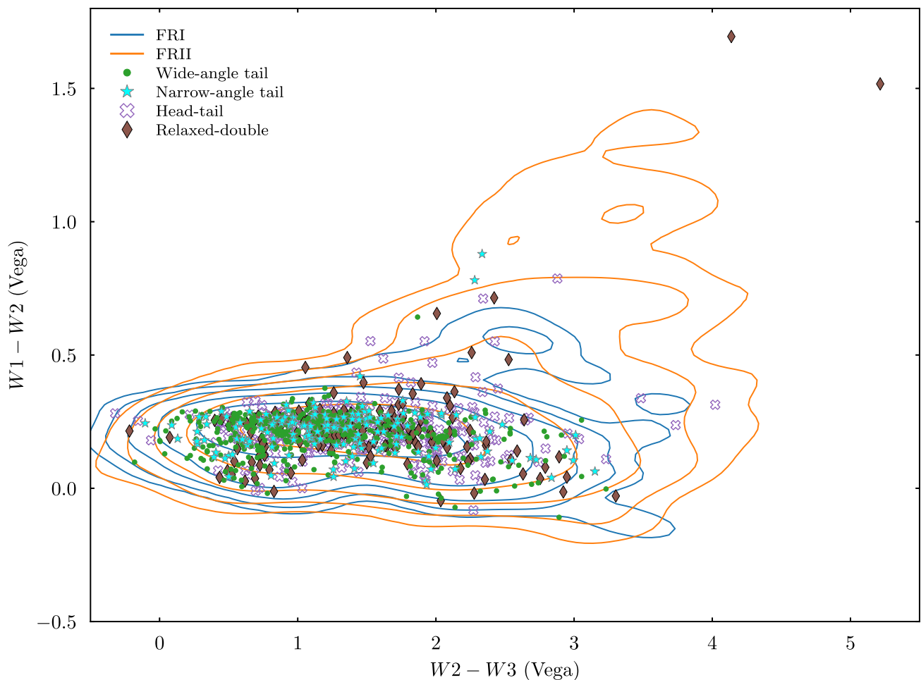
Figure 9. The distribution of various morphological classes within our sample in the WISE colour-colour space. Approximately 50 per cent of our sources have upper limits in W3 . To avoid clutter, we have not included left arrows to indicate that their true positions might be farther to the left than depicted.
