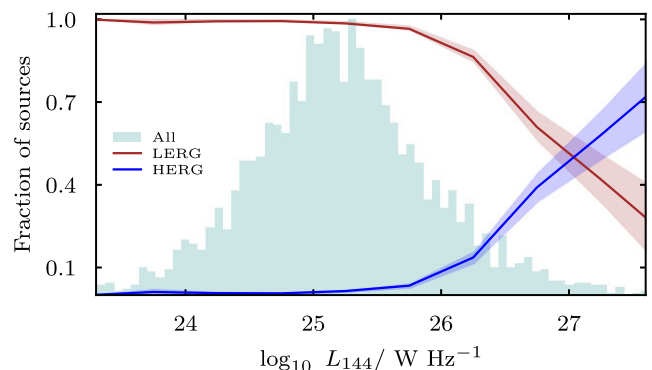
Figure 15. Fraction of low-excitation and high-excitation radio galaxies in our sample as a function of radio luminosity. Shaded regions represent binomial-based errors, indicating the uncertainty in the fraction of sources within each bin of size \Delta \log_{10} L_{144}/\text{W Hz}^{-1} = 0.5 .
