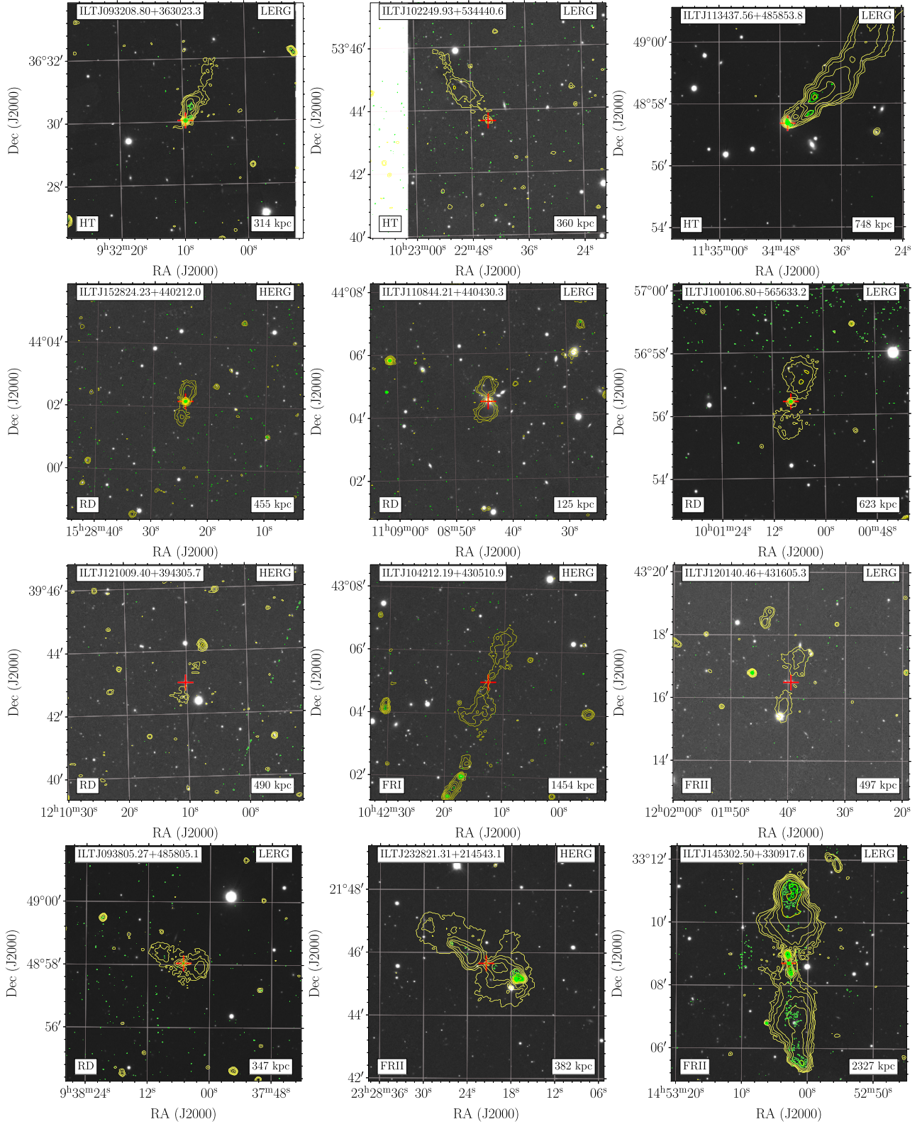
Figure A2. Continued from Fig. A1. The bottom panel shows examples of restarted candidate sources, while the penultimate panel displays remnant candidates. Contours increase logarithmically by factors of 2, starting from 3\sigma .
