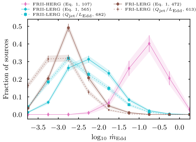
Figure 21. Eddington-scaled accretion rates for the FRII HERG and FRII LERG samples, with the FRI LERG sample included for comparison. Note the difference in the FRII populations in the legend of this plot and Fig. 20; only sources with reliable host mass estimates (see Section 4.3) are shown here. Separate plots are shown for the LERG sample, distinguishing between sources with and without bolometric radiative luminosities estimated from [O III] measurements, as some LERGs lack these measurements. Shaded areas as in Fig. 15.
