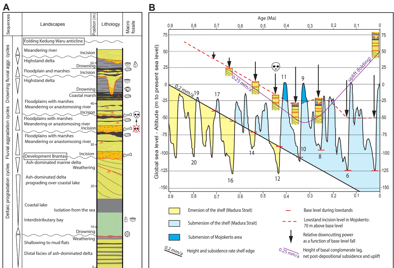
Fig. 1. A: Composite stratigraphic column of the Kedung Waru anticline north of Mojokerto, based on quarry sections east of Kepuhklagen Road. From: Berghuis et al. (2022). Please refer to this paper for detailed facies descriptions. Note the revised stratigraphic level of the Perring Homo erectus skull. B: Reconstruction of successive fluvial cycles in relation to sea-level fluctuations and subsidence. From: Berghuis et al. (2022). Please refer to this paper for more information. Based on the comment by Huffman and Zaim we changed the correlation of the 1936 find level of the Perring skull to the conglomerate lag that forms the base of the third fluvial sequence, suggesting an MIS12 age for the hominin-bearing layer. Sea-level curve based on Bintanja and van de Wal (2008).
