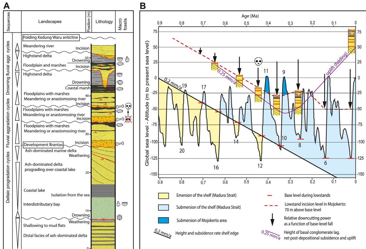
Fig. 1. (A) Composite stratigraphic column of the Kedung Waru anticline north of Mojokerto, based on quarry sections east of Kepuhklagen Road. From: Berghuis et al. (2022). Please refer to this paper for detailed facies descriptions. Note the revised stratigraphic level of the Perning Homo erectus skull. (B) Reconstruction of successive fluvial cycles in relation to sea-level fluctuations and subsidence. From: Berghuis et al. (2022). Please refer to this paper for more information. Based on the comment by Huffman and Zaim we changed the correlation of the 1936 find level of the Perning skull to the conglomerate lag that forms the base of the third fluvial sequence, suggesting an MIS12 age for the hominin-bearing layer. Sea-level curve based on Bintanja and van de Wal (2008).
