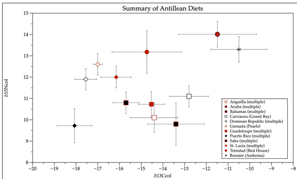
Figure 6. Chart of \delta^{13}\text{C}_{\text{col}} and \delta^{15}\text{N}_{\text{col}} results showing mean values and standard deviation values (arrow bars) for previously published isotope values from Caribbean islands (single or multiple sites mentioned in the parentheses).
