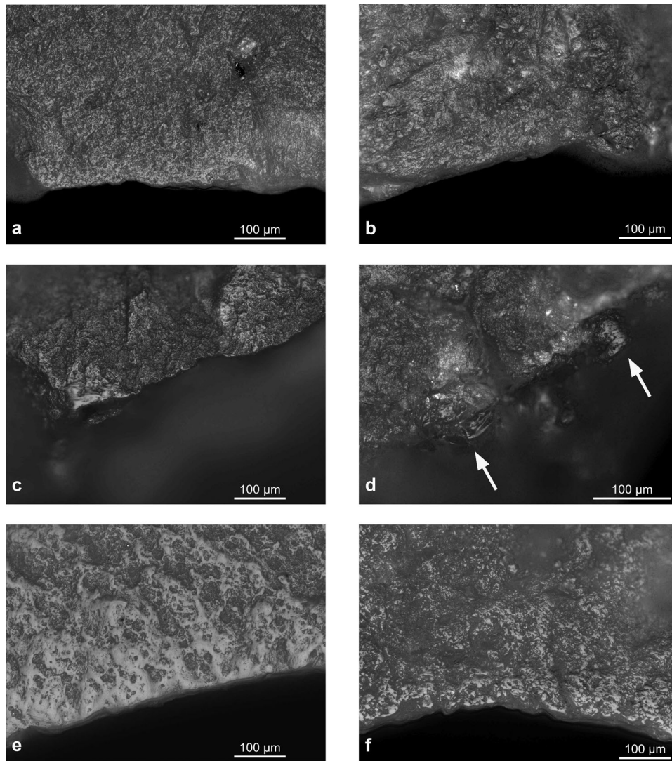
Figure 10. Comparison between polishes on experimental flint tools (a, c, e) and on the unflaked cortical exterior of experimental quartz tools (b, d, f). (a–b) Fresh hide polish. (c–d) Fresh bone polish. (e–f) Fresh reed polish. (a, b, c, e, f) Magnification 200x. (d) Magnification 300x.
