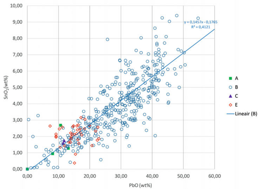
Fig. 13 Biplot of \text{SnO}_2 ratios against \text{PbO} ratios of yellow opaque bead-types.
