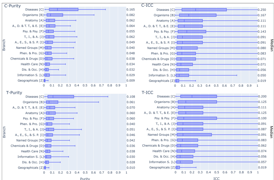
Fig. 1 Box plots showing the distribution of C-Purity, C-ICC, T-Purity and T-ICC over the 45 combinations of parameter values. The median values of each box plot are reported along the right Y axis. The branches are sorted as in Table 3
