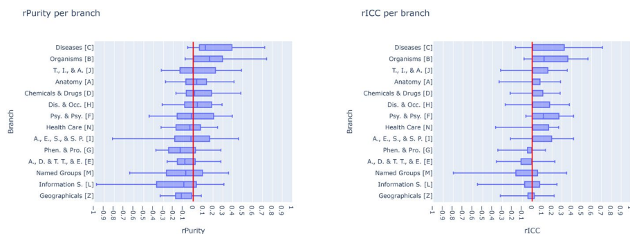
Fig. 3 Box plots showing the distribution of rPurity and rICC for each branch
