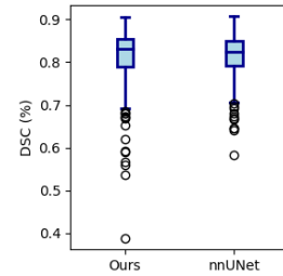
Figure 3.5: Results on the LiVS [24] dataset. Left: The performance of our method compared with HiDiff [42], MERIT [54], TransUNet [55], MedSegDiff [39], EnsemDiff [38], Swin UNETR [2], nnUNet [1] and Gao et al. [24]. ciDice and Con are not applicable for the LiVS dataset with discontinuous annotations. Our method outperforms others in terms of Sen scores. Spe of our model is slightly lower than EnsemDiff , which is a trade-off between completeness ( Sen ) and accuracy ( Spe ) of vessel segmentation. Right: Our DSC score is comparable with nnUNet because high-contrast tumors in the liver cause more outliers (shown in the box plot), negatively affecting the averaged DSC score. Deterministic methods are more efficient than generative methods in inference.
