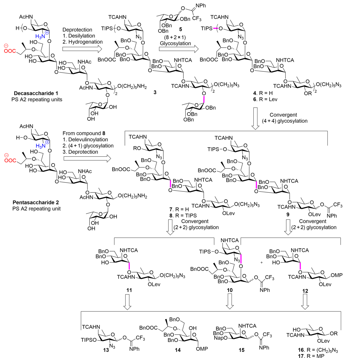
Fig. 2. The retrosynthesis analysis for PS A2 oligosaccharides 1 and 2.
