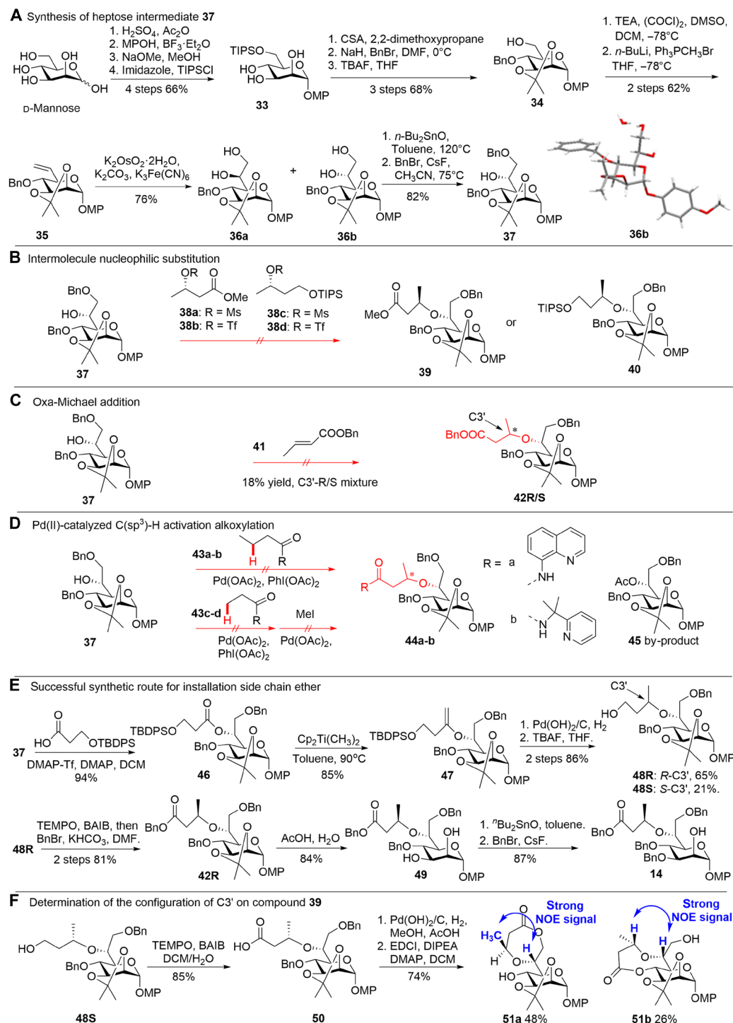
Fig. 4. Synthesis of mannoheptose building block 14. (A) Synthesis of heptose intermediate 37; (B) Intermolecule nucleophilic substitution; (C) Oxa-Michael addition; (D) Pd(II)-catalyzed C(sp 3 )-H activation alkoxylation; (E) Successful synthetic route for installation side chain ether; (F) Determination of the configuration of C3' on compound 39.
