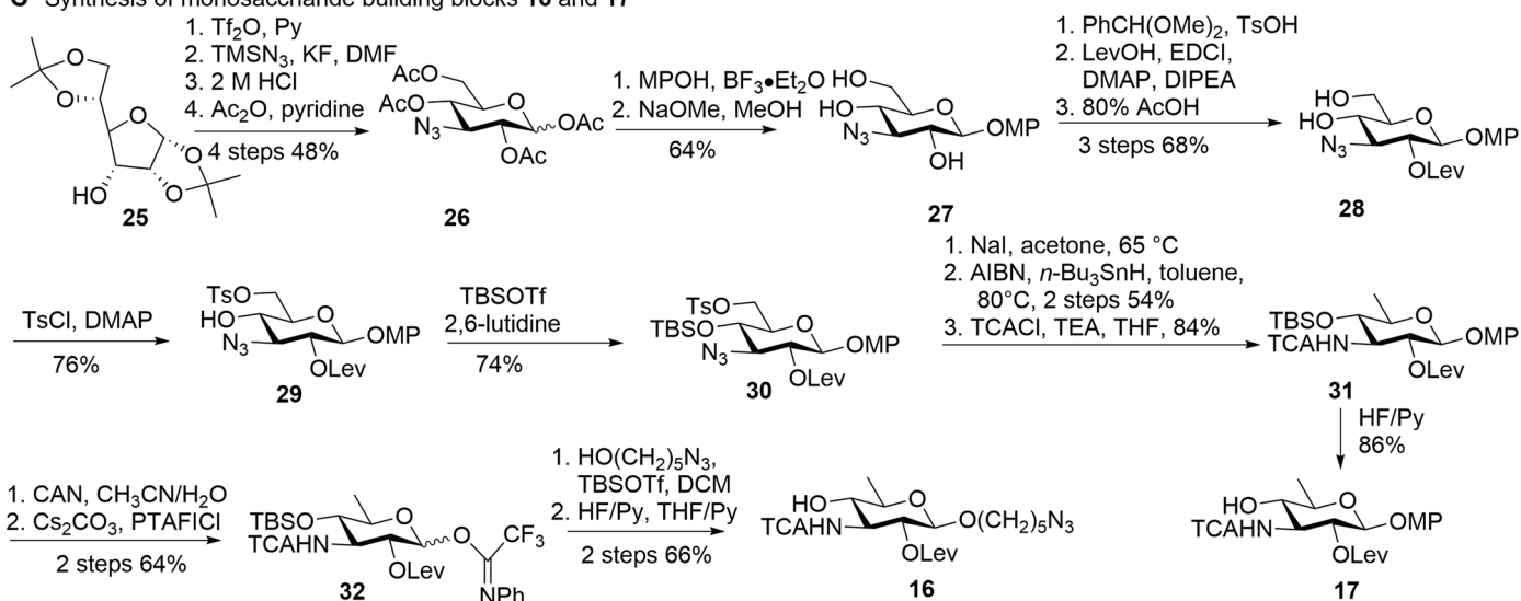
Fig. 3. Synthesis of monosaccharide building blocks 13, 15', 16, and 17. (A) Synthesis of 13; (B) Synthesis of 15'; (C) Synthesis of 16–17.
