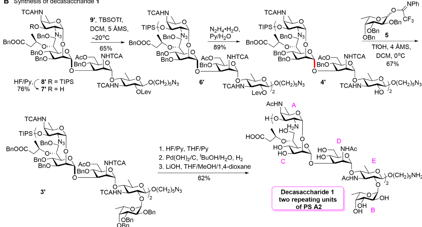
Fig. 6. Synthesis of target decasaccharide 1 containing two repeating units of PS A2. (A) Synthesis of tetrasaccharide donor 9' ; (B) Synthesis of decasaccharide 1 .
