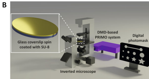
Figure 1. Microfabrication process flow using maskless photolithography. (A) Flowchart showing the developed approach to rapidly fabricate OoC devices. (B) Schematic of DMD-based maskless photolithography setup (PRIMO). (C) Photograph of microfabricated SU-8 mold mounted into a Petri dish (60 mm diameter) for soft lithography.
