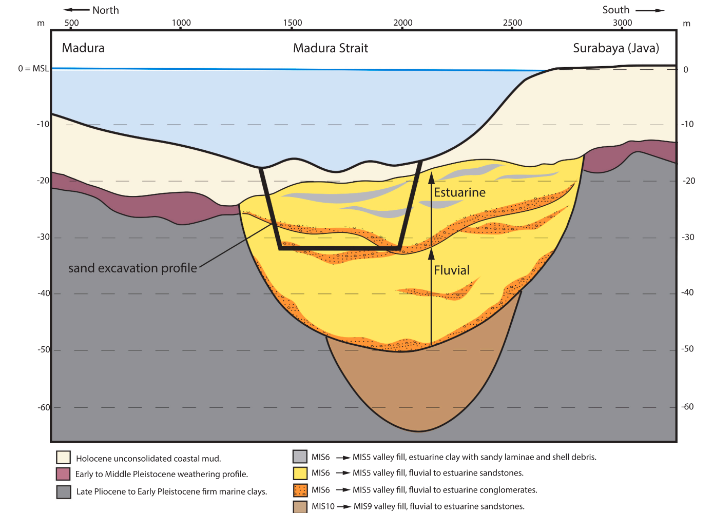
Fig. 2. Schematic cross-section over the Madura Strait north of Surabaya, with a projection of the sand-extraction profile. The local subsoil contains the remnants of two superimposed paleovalleys of the Solo. The extracted material is the sandy fill of the highest paleovalley. Incision of the two paleovalleys has been tied to the lowstands of MIS10 and MIS6 respectively. The valley-fill sequences relate to subsequent transgressive stages. For details, see Berghuis et al. (2025a; 2025c) .
