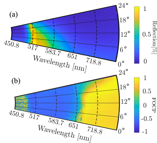
Fig. 4. Angle dependence of the optical properties of Protetia speciosa jousnelini False colour images of the reflectance (a) and Fraction of circular polarization (b) plotted as function of angle of incidence and wavelength.
