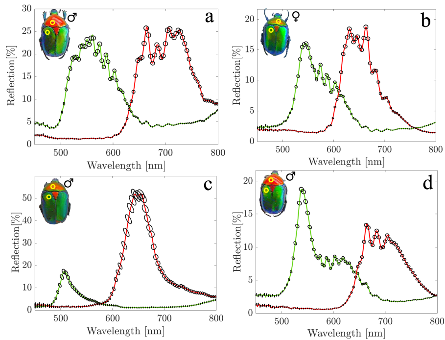
Fig. 3. Polarization resolved hyperspectral imaging of Protetia speciosa jousseini beetles (a)-(d) Reflectance spectra of two distinct parts of the beetles (elytra, (green curves) and pronotum, (red curves)). The ellipses refer to the elliptical polarization state as a function of wavelength. The insets show images of each beetle with yellow circles indicating the locations where the spectra shown in the main figure are extracted.
