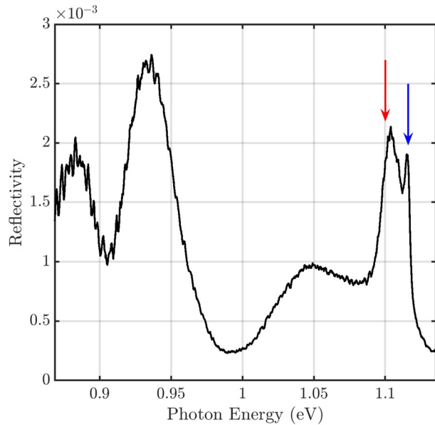
Figure 7: Spectrum in the center of the cavity for \hat{E}_{\text{in}} = \hat{V} and \hat{E}_{\text{out}} = \hat{H} . This configuration is symmetry-forbidden. The blue arrow marks the resonance energy of the high- Q mode, the red arrow of the low- Q mode (cf. Fig. A.1 and Fig. A.2).
