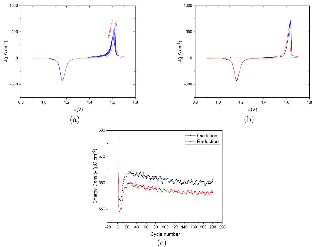
Figure 7. (a) Cyclic voltammograms of the consecutively applied 200 ORCs on Au(111) in 0.1 M H 2 SO 4 and 1 μM HCl with a scan rate of 50 mV s -1 vs RHE. The color spectrum ranges from blue for the first cycle to red for the last cycle. The arrows show the trajectory of the oxidation peak. (b) First and last cycle in blue and red, respectively, for a better representation. (c) Calculated oxidation (black) and reduction (red) charge density (μC cm -2 ) vs cycle number for the CVs shown in (a).
