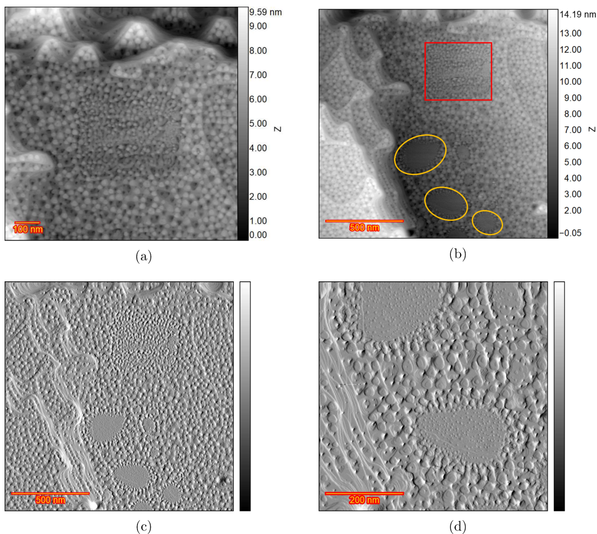
Figure 6. Au(111) in \text{H}_2\text{SO}_4 and 1 \mu\text{M} HCl after 200 ORCs. (a) Large scan area which includes the initial scan area at the center. (b) Further zoomed-out frame which contains the initial scan area and some spots with no roughening. (c) The differential image of the frame shown in (b). (d) Zoomed-in image of the spots with no roughening.
