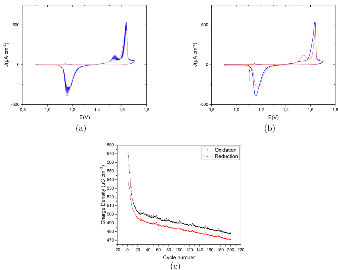
Figure 4. (a) Cyclic voltammograms of the consecutively applied 200 ORCs on Au(111) in 0.1 M H 2 SO 4 and 10 μM HCl with a scan rate of 50 mV s −1 vs RHE. The color spectrum ranges from blue for the first cycle to red for the last cycle. (b) First and last cycle in blue and red, respectively, for a better representation. (c) Calculated oxidation (black) and reduction (red) charge density (μC cm −2 ) vs cycle number for the CVs shown in (a).
