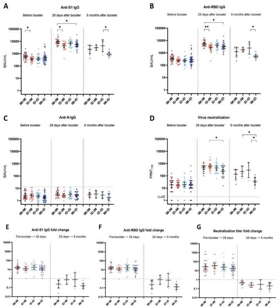
Figure 2. Antibody responses
