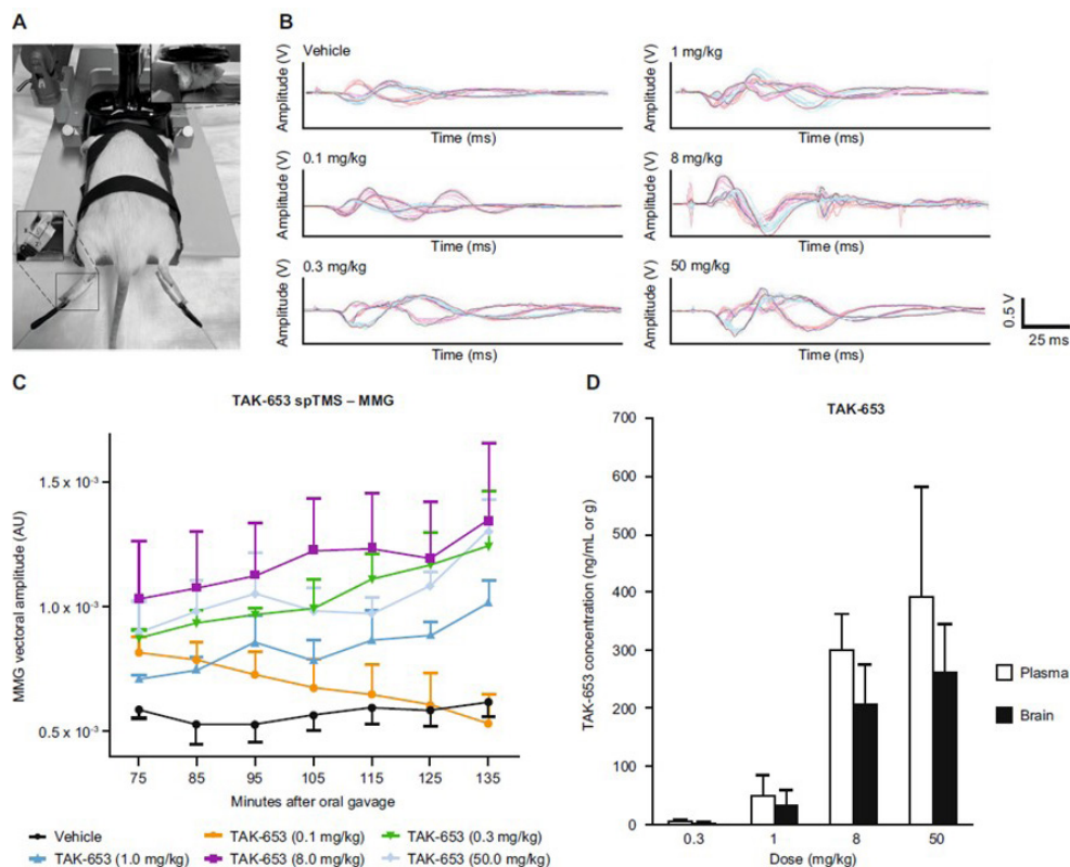
Figure 1 TAK-653 enhanced TMS-evoked motor responses in rats
