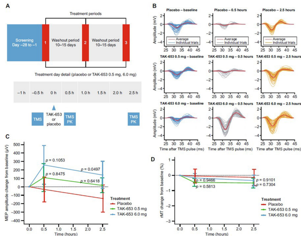
A. Study schematic (top) and detail of treatment day events (bottom). B. Representative MEP waveforms from one participant at baseline, 30 minutes, and 2.5 hours post-dose for all three treatment periods. C. Changes from baseline in MEP amplitude for placebo, 0.5 mg TAK-653, and 6 mg TAK-653 periods. p = Dunnett's adjusted p value. D. Changes from baseline in rMT for all three periods. MEP, motor-evoked potentials; PK, pharmacokinetic; rMT, resting motor threshold; TMS, transcranial magnetic stimulation.
