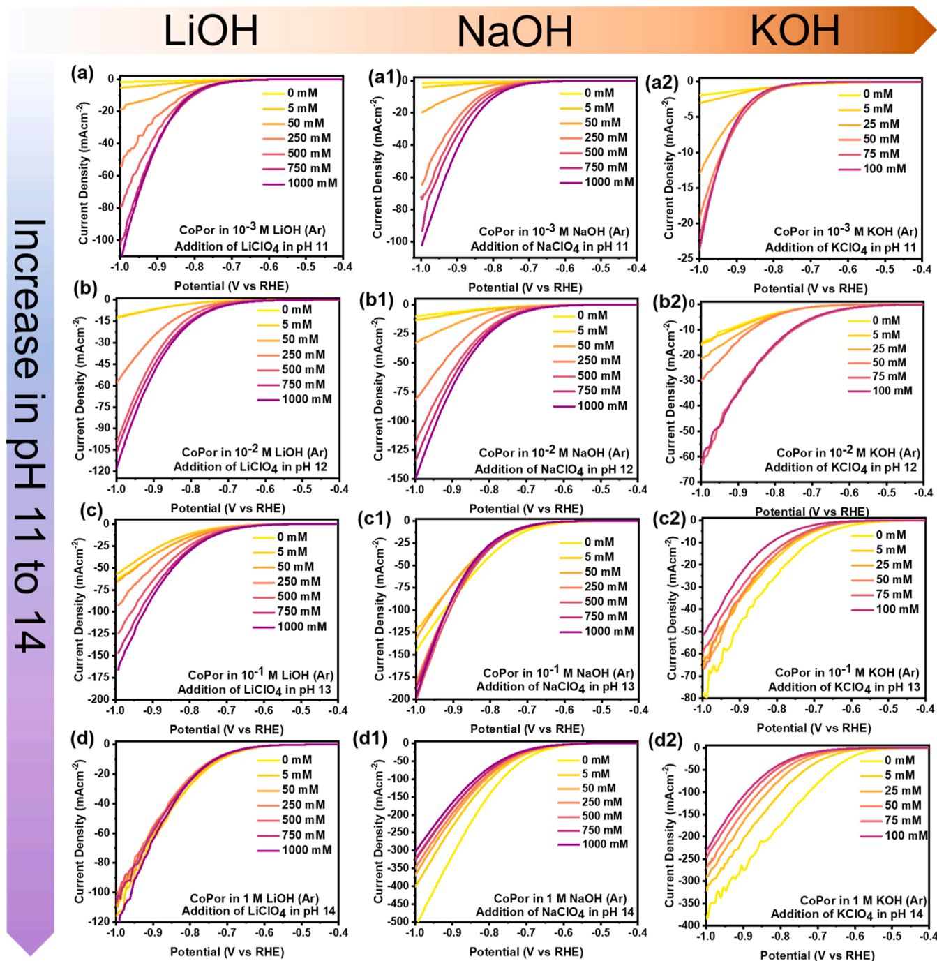
Fig. 3. HER polarization curves recorded on the 0.6 m cm -2 loading of CoPor on RDE rotating at a rotation of 1600 RPM in Ar-saturated MOH solutions. LSVs at the scan rate of 20 mV s -1 recorded in (a-d) LiOH-based electrolytes, (a1-d1) NaOH-based electrolytes and (a2-d2) KOH-based electrolytes. To analyze the effects of AMs + concentrations, LiClO 4 and NaClO 4 were sequentially added up to 1000 mM concentrations in LiOH and NaOH-based solutions, respectively, whereas KClO 4 was added to a maximum concentration of 100 mM due to its solubility limit.
