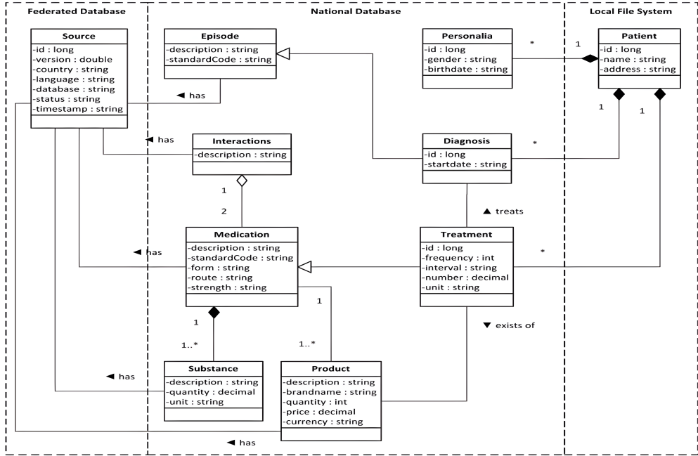
Figure 2.1: Class Diagram depicting main data models of STRIPA
